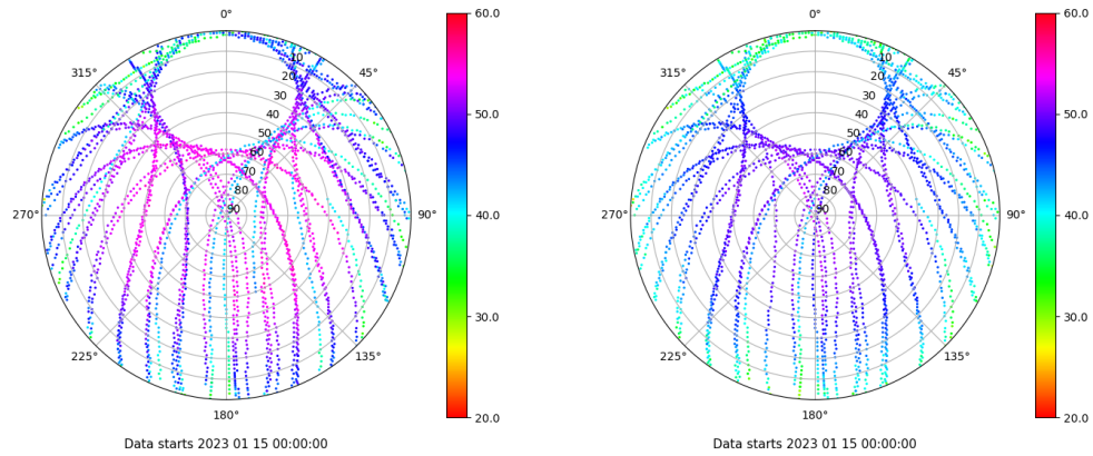
Skyplot for station VALA. Signal to Noise S1C Data file VALA00ESP_R_2023015.xtr Skyplot for station VALA. Signal to Noise S2C Data file VALA00ESP_R_2023015.xtr
