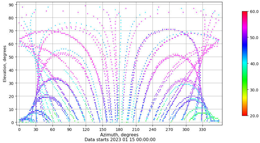
Azimuth-elevation plot for station VALA. Signal to Noise S1C Data file VALA00ESP_R_2023015.xtr
