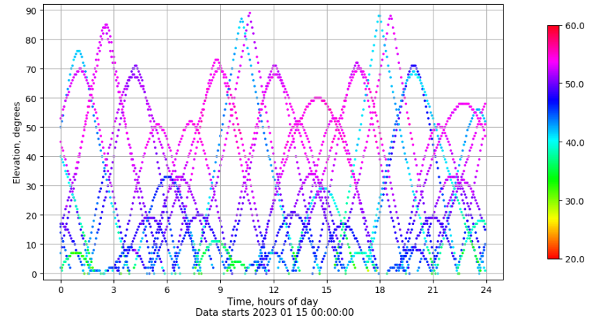
Time-elevation plot for station VALA. Signal to Noise S1C Data file VALA00ESP_R_2023015.xtr
