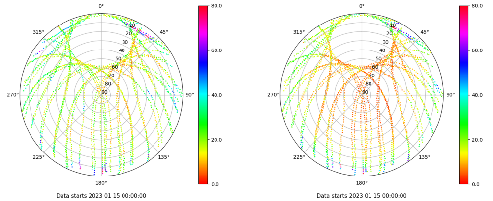
Skyplot for station VALA. Parameter M1C Data file VALA00ESP_R_2023015.xtr Skyplot for station VALA. Parameter M2C Data file VALA00ESP_R_2023015.xtr
