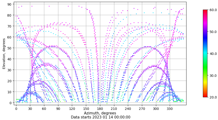
Azimuth-elevation plot for station VALA. Signal to Noise S1C Data file VALA00ESP_R_2023014.xtr
