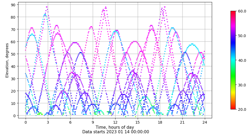
Time-elevation plot for station VALA. Signal to Noise S1C Data file VALA00ESP_R_2023014.xtr
