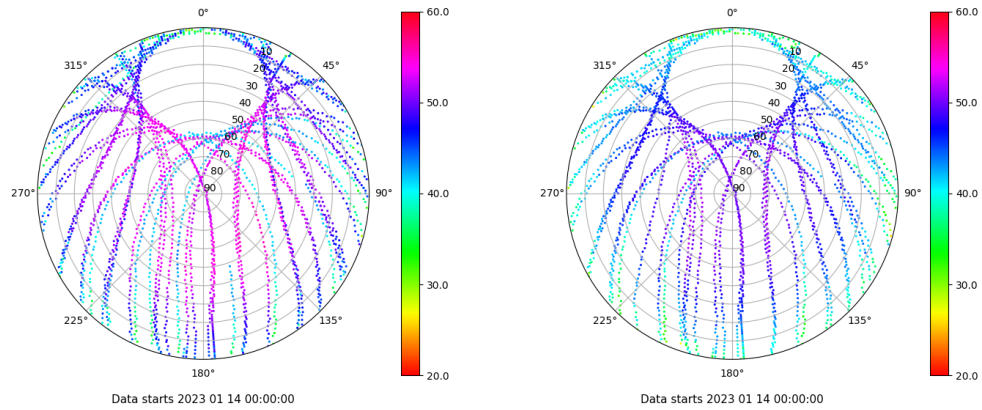
Skyplot for station VALA. Signal to Noise S1C Data file VALA00ESP_R_2023014.xtr Skyplot for station VALA. Signal to Noise S2C Data file VALA00ESP_R_2023014.xtr
