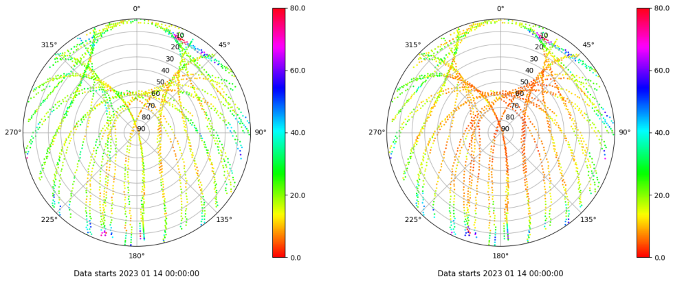
Skyplot for station VALA. Parameter M1C Data file VALA00ESP_R_2023014.xtr Skyplot for station VALA. Parameter M2C Data file VALA00ESP_R_2023014.xtr
