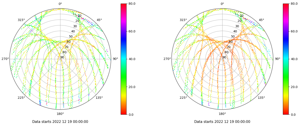
Skyplot for station VALA. Parameter M1C Data file VALA00ESP_R_2022353.xtr Skyplot for station VALA. Parameter M2C Data file VALA00ESP_R_2022353.xtr
