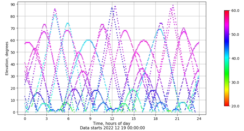
Time-elevation plot for station VALA. Signal to Noise S1C Data file VALA00ESP_R_2022353.xtr
