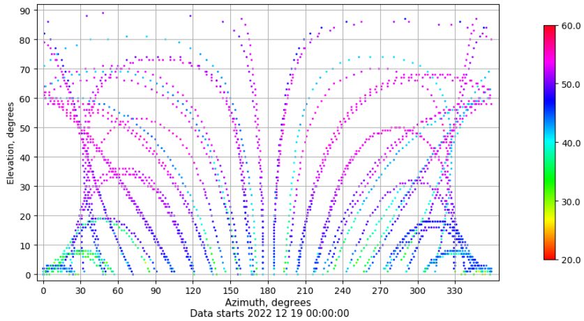
Azimuth-elevation plot for station VALA. Signal to Noise S1C Data file VALA00ESP_R_2022353.xtr
