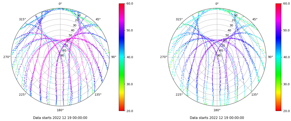
Skyplot for station VALA. Signal to Noise S1C Data file VALA00ESP_R_2022353.xtr Skyplot for station VALA. Signal to Noise S2C Data file VALA00ESP_R_2022353.xtr
