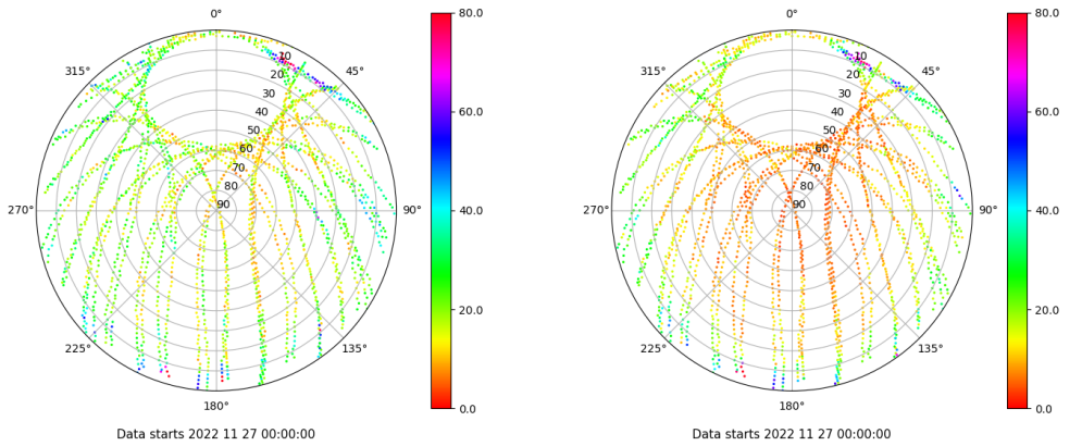
Skyplot for station VALA. Parameter M1C Data file VALA00ESP_R_2022331.xtr Skyplot for station VALA. Parameter M2C Data file VALA00ESP_R_2022331.xtr
