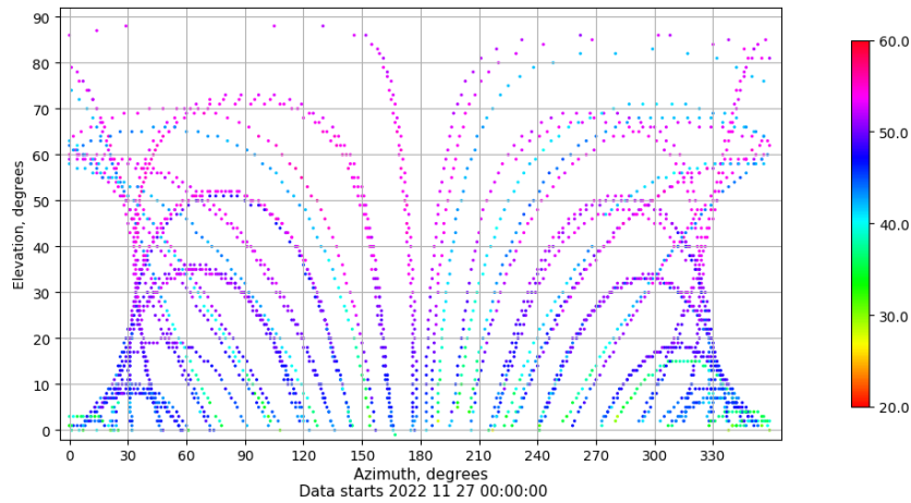
Azimuth-elevation plot for station VALA. Signal to Noise S1C Data file VALA00ESP_R_2022331.xtr
