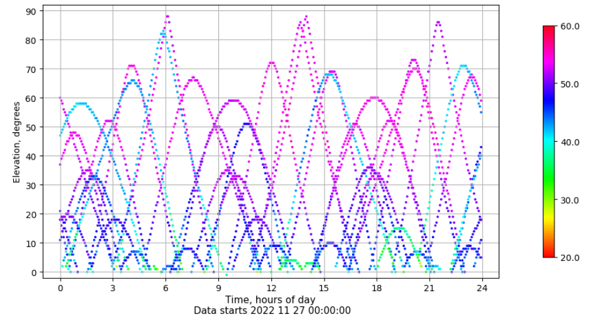
Time-elevation plot for station VALA. Signal to Noise S1C Data file VALA00ESP_R_2022331.xtr
