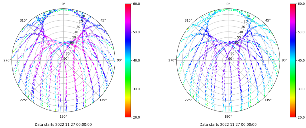
Skyplot for station VALA. Signal to Noise S1C Data file VALA00ESP_R_2022331.xtr Skyplot for station VALA. Signal to Noise S2C Data file VALA00ESP_R_2022331.xtr
