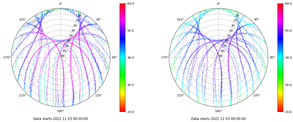
Skyplot for station VALA. Signal to Noise S1C Data file VALA00ESP_R_2022307.xtr Skyplot for station VALA. Signal to Noise S2C Data file VALA00ESP_R_2022307.xtr
