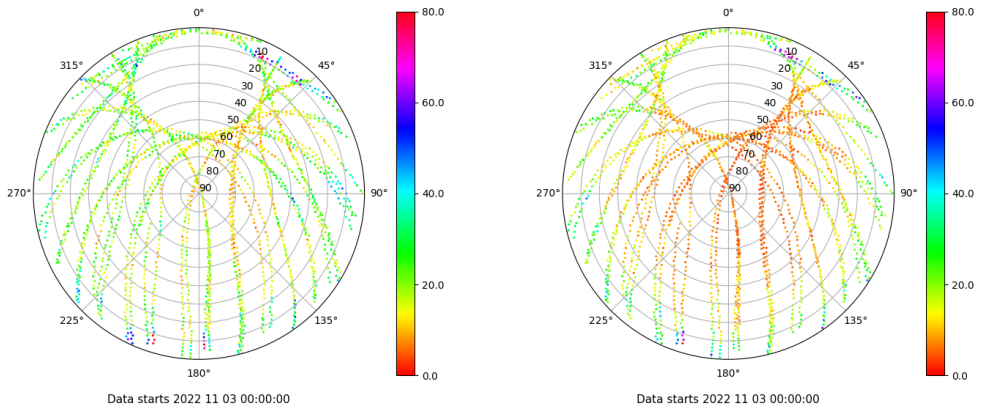
Skyplot for station VALA. Parameter M1C Data file VALA00ESP_R_2022307.xtr Skyplot for station VALA. Parameter M2C Data file VALA00ESP_R_2022307.xtr
