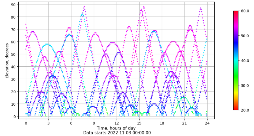
Time-elevation plot for station VALA. Signal to Noise S1C Data file VALA00ESP_R_2022307.xtr
