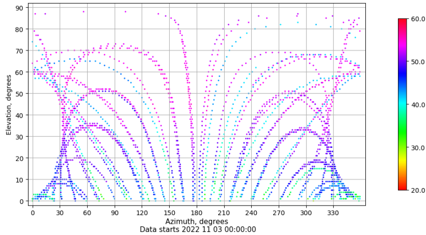
Azimuth-elevation plot for station VALA. Signal to Noise S1C Data file VALA00ESP_R_2022307.xtr
