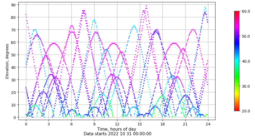
Time-elevation plot for station VALA. Signal to Noise S1C Data file VALA00ESP_R_2022304.xtr
