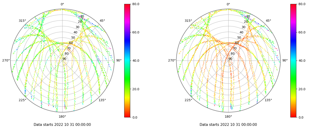
Skyplot for station VALA. Parameter M1C Data file VALA00ESP_R_2022304.xtr Skyplot for station VALA. Parameter M2C Data file VALA00ESP_R_2022304.xtr
