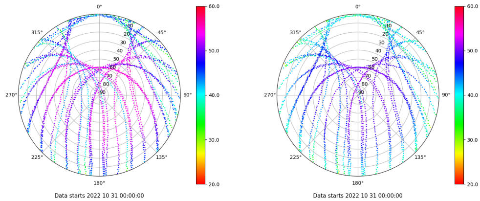
Skyplot for station VALA. Signal to Noise S1C Data file VALA00ESP_R_2022304.xtr Skyplot for station VALA. Signal to Noise S2C Data file VALA00ESP_R_2022304.xtr
