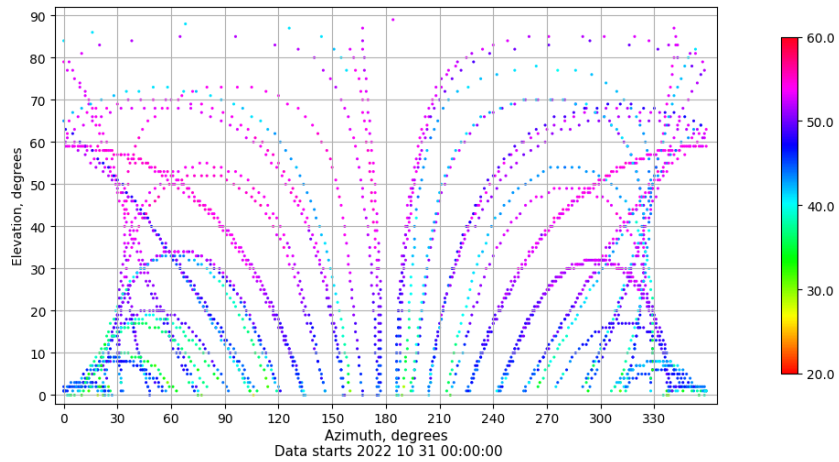
Azimuth-elevation plot for station VALA. Signal to Noise S1C Data file VALA00ESP_R_2022304.xtr
