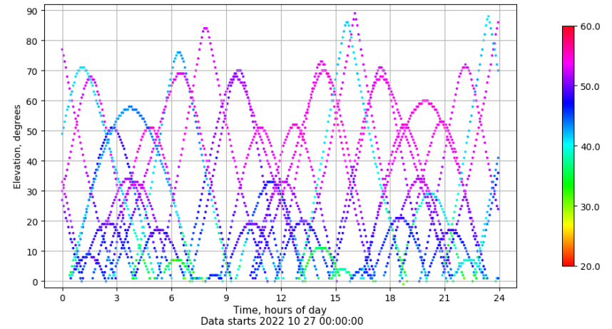
Time-elevation plot for station VALA. Signal to Noise S1C Data file VALA00ESP_R_2022300.xtr
