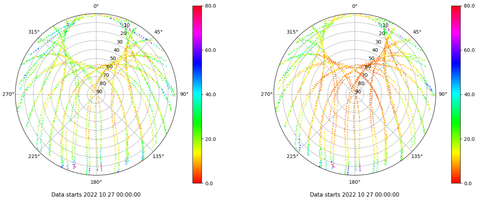
Skyplot for station VALA. Parameter M1C Data file VALA00ESP_R_2022300.xtr Skyplot for station VALA. Parameter M2C Data file VALA00ESP_R_2022300.xtr
