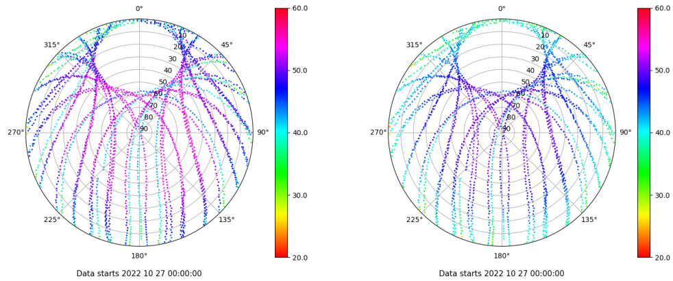
Skyplot for station VALA. Signal to Noise S1C Data file VALA00ESP_R_2022300.xtr Skyplot for station VALA. Signal to Noise S2C Data file VALA00ESP_R_2022300.xtr
