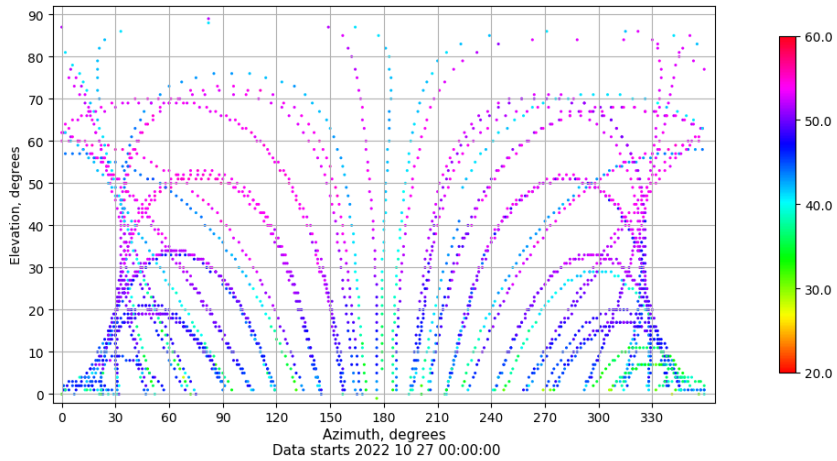
Azimuth-elevation plot for station VALA. Signal to Noise S1C Data file VALA00ESP_R_2022300.xtr
