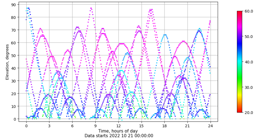
Time-elevation plot for station VALA. Signal to Noise S1C Data file VALA00ESP_R_2022294.xtr
