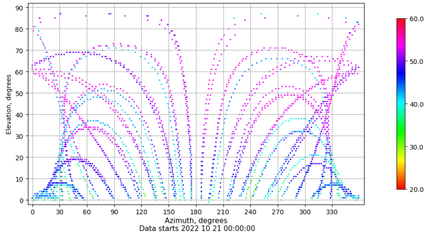
Azimuth-elevation plot for station VALA. Signal to Noise S1C Data file VALA00ESP_R_2022294.xtr
