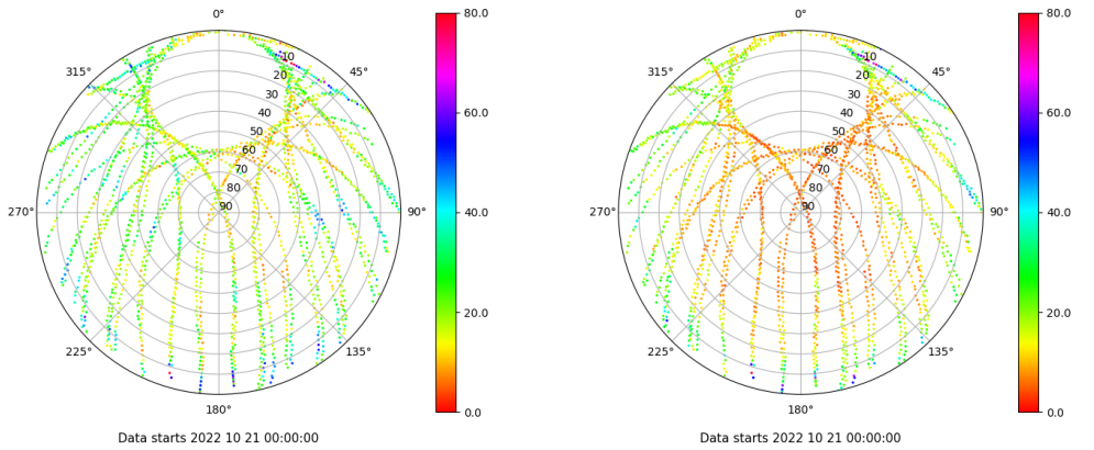
Skyplot for station VALA. Parameter M1C Data file VALA00ESP_R_2022294.xtr Skyplot for station VALA. Parameter M2C Data file VALA00ESP_R_2022294.xtr
