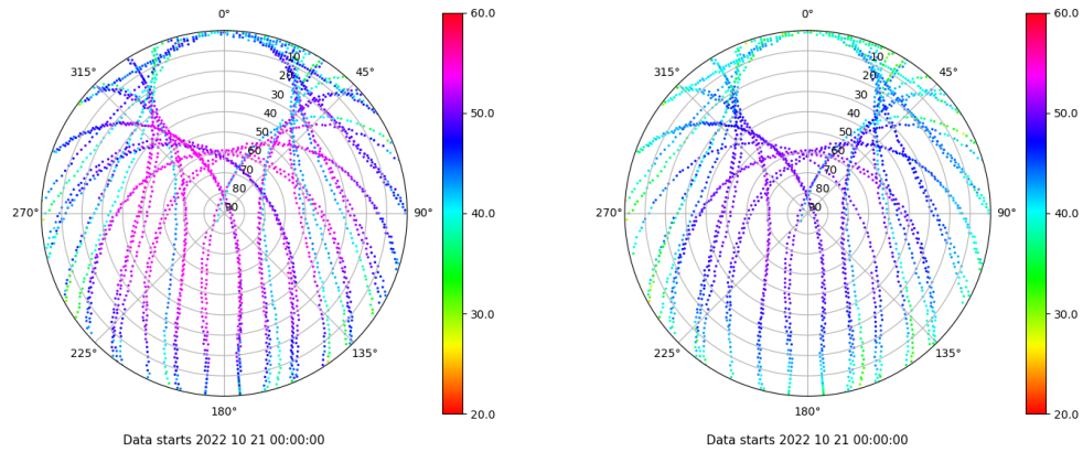
Skyplot for station VALA. Signal to Noise S1C Data file VALA00ESP_R_2022294.xtr Skyplot for station VALA. Signal to Noise S2C Data file VALA00ESP_R_2022294.xtr
