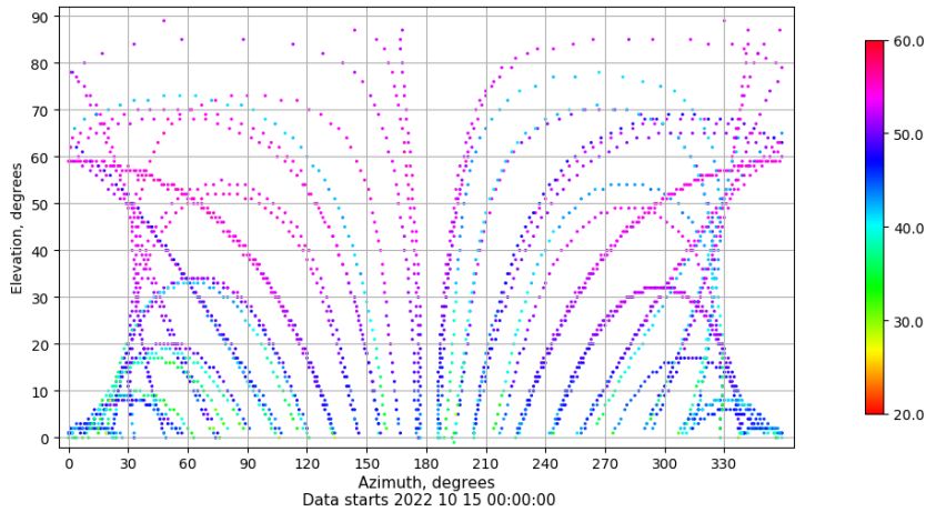
Azimuth-elevation plot for station VALA. Signal to Noise S1C Data file VALA00ESP_R_2022288.xtr
