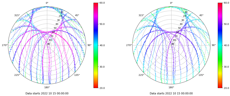
Skyplot for station VALA. Signal to Noise S1C Data file VALA00ESP_R_2022288.xtr Skyplot for station VALA. Signal to Noise S2C Data file VALA00ESP_R_2022288.xtr
