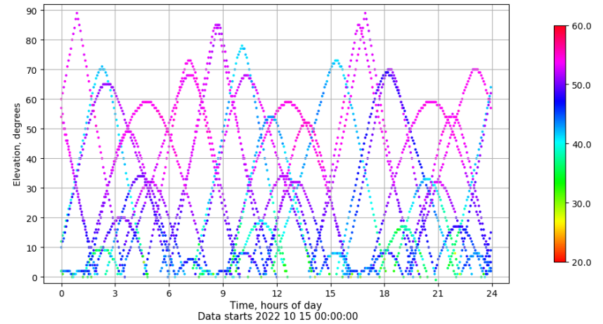
Time-elevation plot for station VALA. Signal to Noise S1C Data file VALA00ESP_R_2022288.xtr
