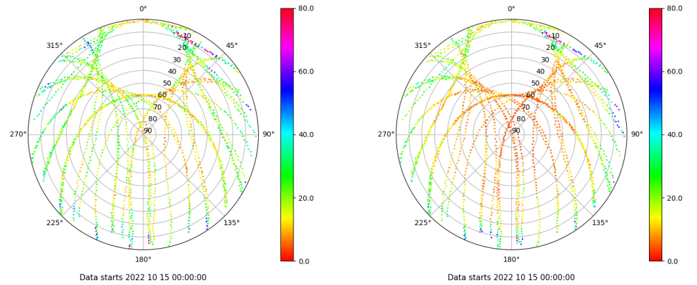
Skyplot for station VALA. Parameter M1C Data file VALA00ESP_R_2022288.xtr Skyplot for station VALA. Parameter M2C Data file VALA00ESP_R_2022288.xtr
