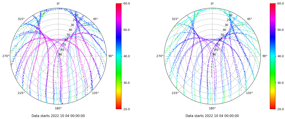
Skyplot for station VALA. Signal to Noise S1C Data file VALA00ESP_R_2022277.xtr Skyplot for station VALA. Signal to Noise S2C Data file VALA00ESP_R_2022277.xtr
