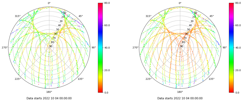
Skyplot for station VALA. Parameter M1C Data file VALA00ESP_R_2022277.xtr Skyplot for station VALA. Parameter M2C Data file VALA00ESP_R_2022277.xtr
