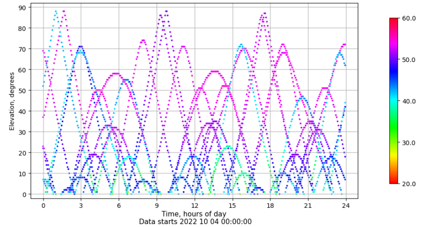
Time-elevation plot for station VALA. Signal to Noise S1C Data file VALA00ESP_R_2022277.xtr
