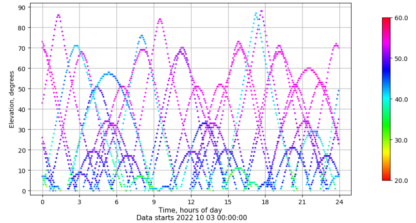
Time-elevation plot for station VALA. Signal to Noise S1C Data file VALA00ESP_R_2022276.xtr
