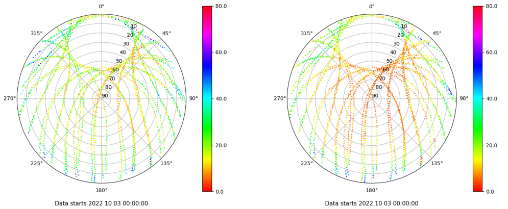
Skyplot for station VALA. Parameter M1C Data file VALA00ESP_R_2022276.xtr Skyplot for station VALA. Parameter M2C Data file VALA00ESP_R_2022276.xtr
