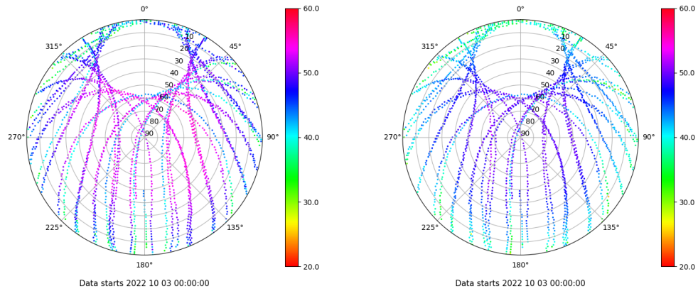
Skyplot for station VALA. Signal to Noise S1C Data file VALA00ESP_R_2022276.xtr Skyplot for station VALA. Signal to Noise S2C Data file VALA00ESP_R_2022276.xtr
