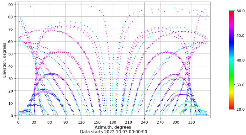
Azimuth-elevation plot for station VALA. Signal to Noise S1C Data file VALA00ESP_R_2022276.xtr
