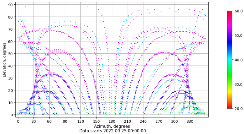
Azimuth-elevation plot for station VALA. Signal to Noise S1C Data file VALA00ESP_R_2022268.xtr
