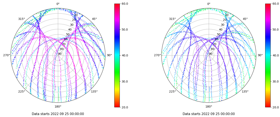
Skyplot for station VALA. Signal to Noise S1C Data file VALA00ESP_R_2022268.xtr Skyplot for station VALA. Signal to Noise S2C Data file VALA00ESP_R_2022268.xtr
