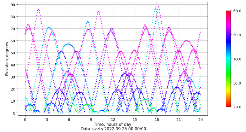
Time-elevation plot for station VALA. Signal to Noise S1C Data file VALA00ESP_R_2022268.xtr
