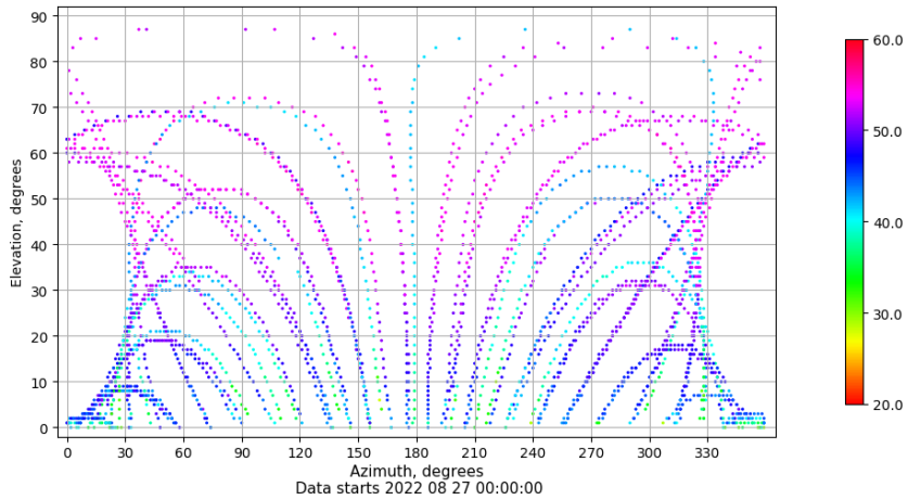
Azimuth-elevation plot for station VALA. Signal to Noise S1C Data file VALA00ESP_R_2022239.xtr
