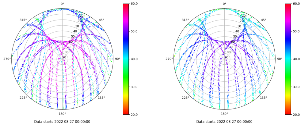
Skyplot for station VALA. Signal to Noise S1C Data file VALA00ESP_R_2022239.xtr Skyplot for station VALA. Signal to Noise S2C Data file VALA00ESP_R_2022239.xtr
