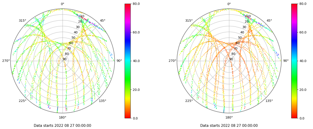
Skyplot for station VALA. Parameter M1C Data file VALA00ESP_R_2022239.xtr Skyplot for station VALA. Parameter M2C Data file VALA00ESP_R_2022239.xtr
