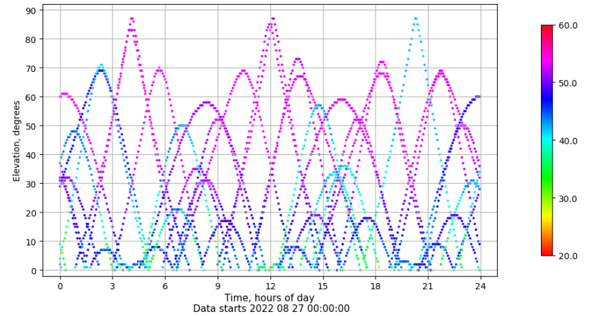
Time-elevation plot for station VALA. Signal to Noise S1C Data file VALA00ESP_R_2022239.xtr
