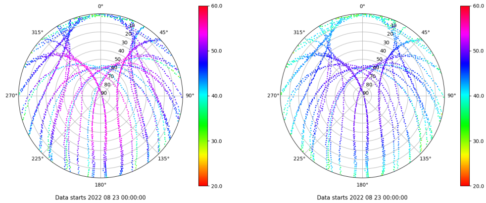
Skyplot for station VALA. Signal to Noise S1C Data file VALA00ESP_R_2022235.xtr Skyplot for station VALA. Signal to Noise S2C Data file VALA00ESP_R_2022235.xtr
