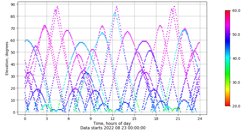
Time-elevation plot for station VALA. Signal to Noise S1C Data file VALA00ESP_R_2022235.xtr
