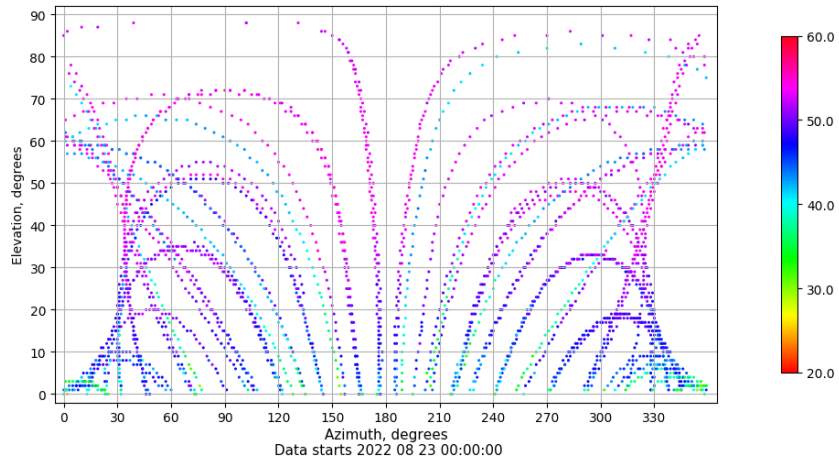
Azimuth-elevation plot for station VALA. Signal to Noise S1C Data file VALA00ESP_R_2022235.xtr
