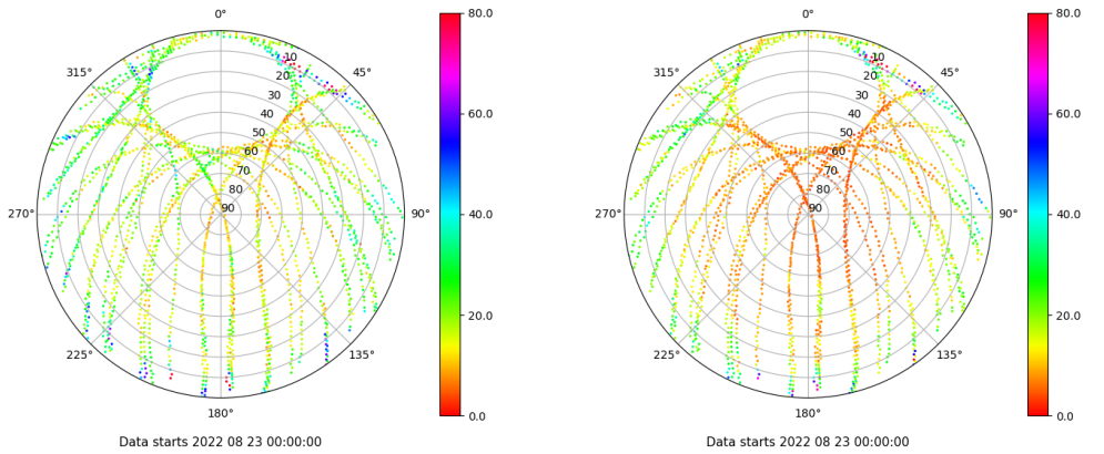
Skyplot for station VALA. Parameter M1C Data file VALA00ESP_R_2022235.xtr Skyplot for station VALA. Parameter M2C Data file VALA00ESP_R_2022235.xtr
