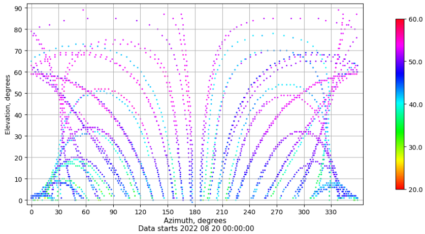
Azimuth-elevation plot for station VALA. Signal to Noise S1C Data file VALA00ESP_R_2022232.xtr
