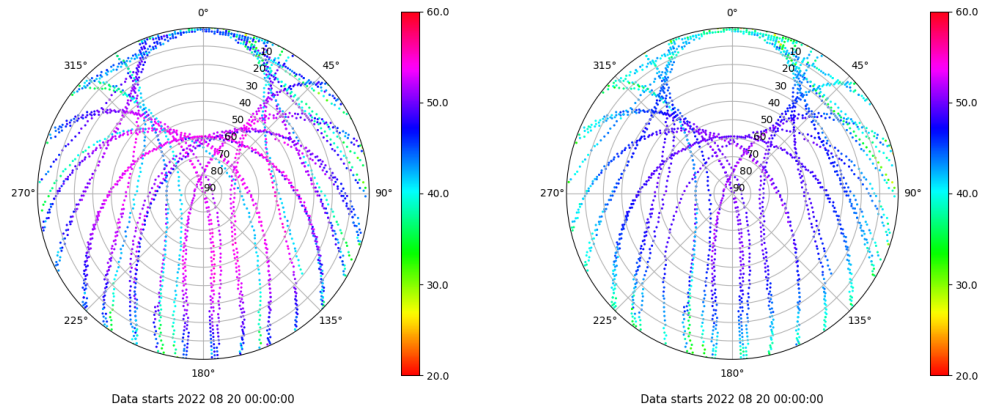
Skyplot for station VALA. Signal to Noise S1C Data file VALA00ESP_R_2022232.xtr Skyplot for station VALA. Signal to Noise S2C Data file VALA00ESP_R_2022232.xtr
