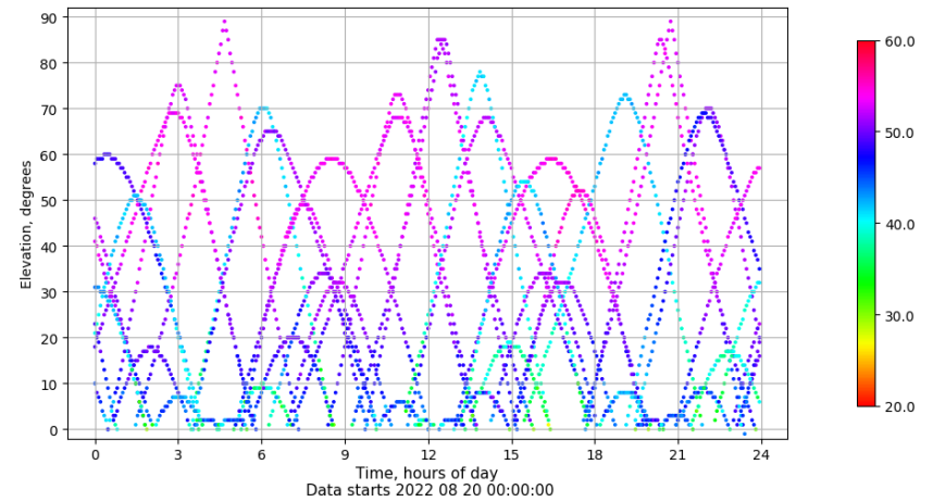
Time-elevation plot for station VALA. Signal to Noise S1C Data file VALA00ESP_R_2022232.xtr
