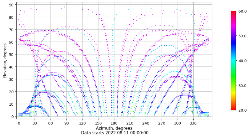
Azimuth-elevation plot for station VALA. Signal to Noise S1C Data file VALA00ESP_R_2022223.xtr
