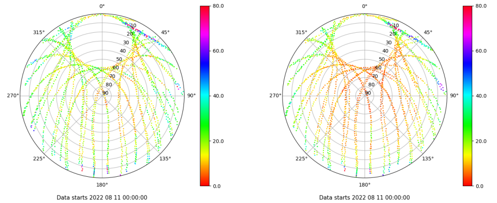
Skyplot for station VALA. Parameter M1C Data file VALA00ESP_R_2022223.xtr Skyplot for station VALA. Parameter M2C Data file VALA00ESP_R_2022223.xtr
