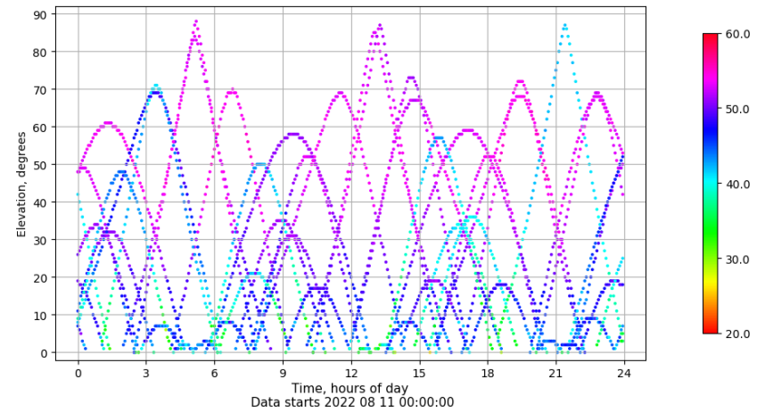
Time-elevation plot for station VALA. Signal to Noise S1C Data file VALA00ESP_R_2022223.xtr
