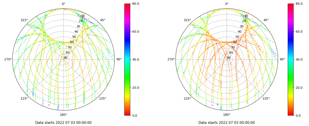
Skyplot for station VALA. Parameter M1C Data file VALA00ESP_R_2022184.xtr Skyplot for station VALA. Parameter M2C Data file VALA00ESP_R_2022184.xtr
