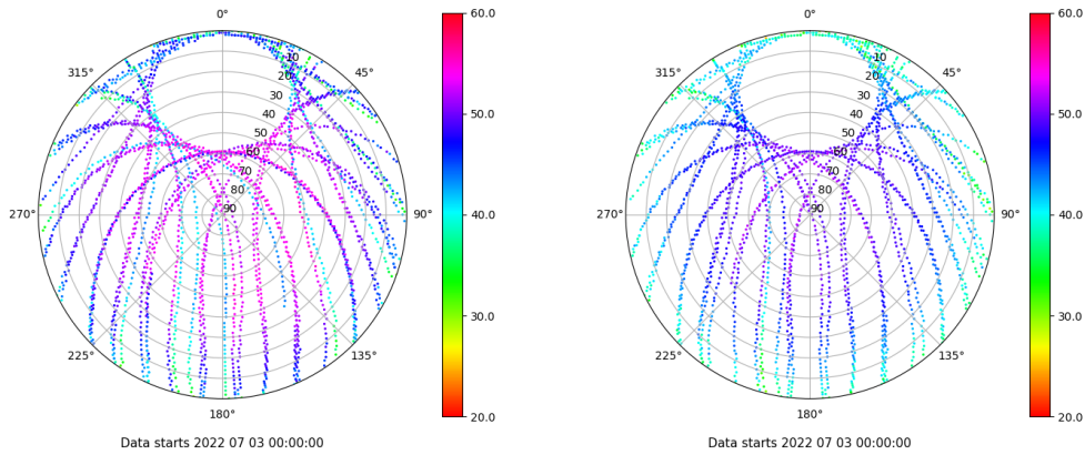
Skyplot for station VALA. Signal to Noise S1C Data file VALA00ESP_R_2022184.xtr Skyplot for station VALA. Signal to Noise S2C Data file VALA00ESP_R_2022184.xtr
