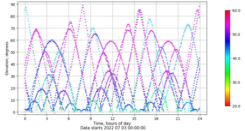
Time-elevation plot for station VALA. Signal to Noise S1C Data file VALA00ESP_R_2022184.xtr
