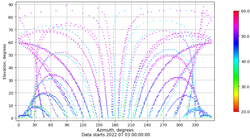
Azimuth-elevation plot for station VALA. Signal to Noise S1C Data file VALA00ESP_R_2022184.xtr
