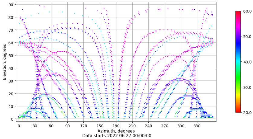
Azimuth-elevation plot for station VALA. Signal to Noise S1C Data file VALA00ESP_R_2022178.xtr
