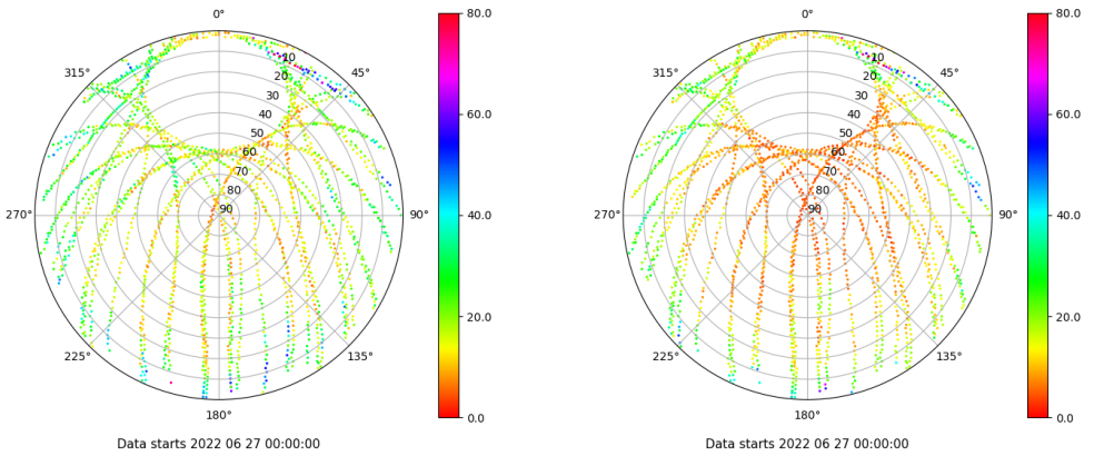
Skyplot for station VALA. Parameter M1C Data file VALA00ESP_R_2022178.xtr Skyplot for station VALA. Parameter M2C Data file VALA00ESP_R_2022178.xtr
