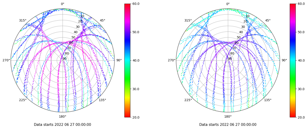
Skyplot for station VALA. Signal to Noise S1C Data file VALA00ESP_R_2022178.xtr Skyplot for station VALA. Signal to Noise S2C Data file VALA00ESP_R_2022178.xtr
