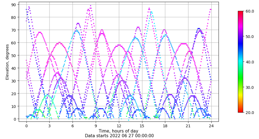
Time-elevation plot for station VALA. Signal to Noise S1C Data file VALA00ESP_R_2022178.xtr
