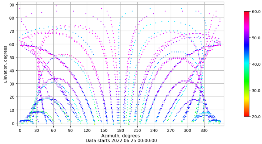
Azimuth-elevation plot for station VALA. Signal to Noise S1C Data file VALA00ESP_R_2022176.xtr
