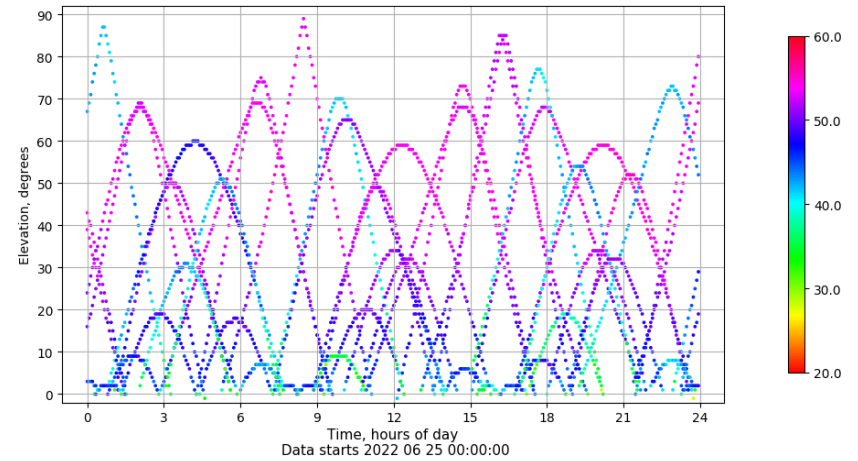
Time-elevation plot for station VALA. Signal to Noise S1C Data file VALA00ESP_R_2022176.xtr
