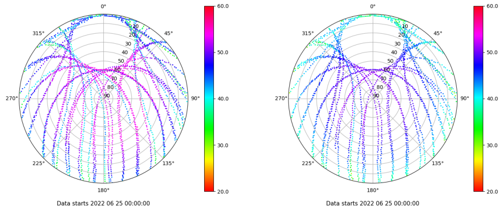
Skyplot for station VALA. Signal to Noise S1C Data file VALA00ESP_R_2022176.xtr Skyplot for station VALA. Signal to Noise S2C Data file VALA00ESP_R_2022176.xtr
