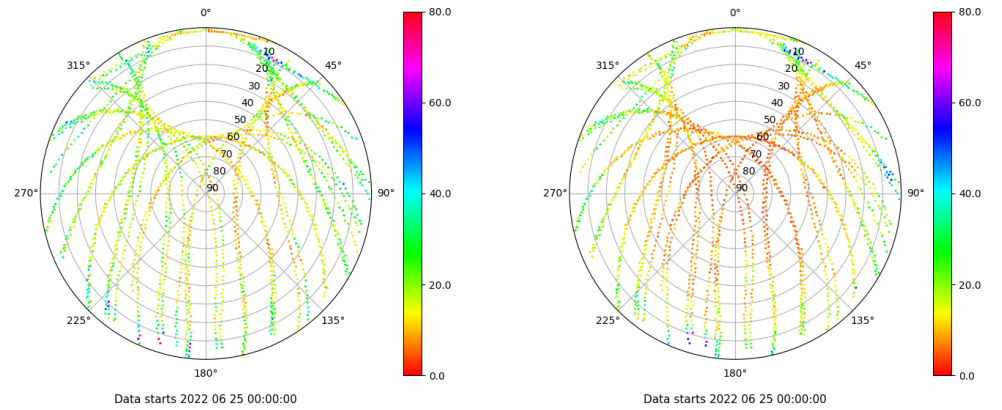
Skyplot for station VALA. Parameter M1C Data file VALA00ESP_R_2022176.xtr Skyplot for station VALA. Parameter M2C Data file VALA00ESP_R_2022176.xtr
