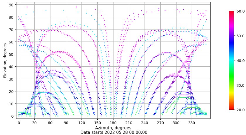
Azimuth-elevation plot for station VALA. Signal to Noise S1C Data file VALA00ESP_R_2022148.xtr
