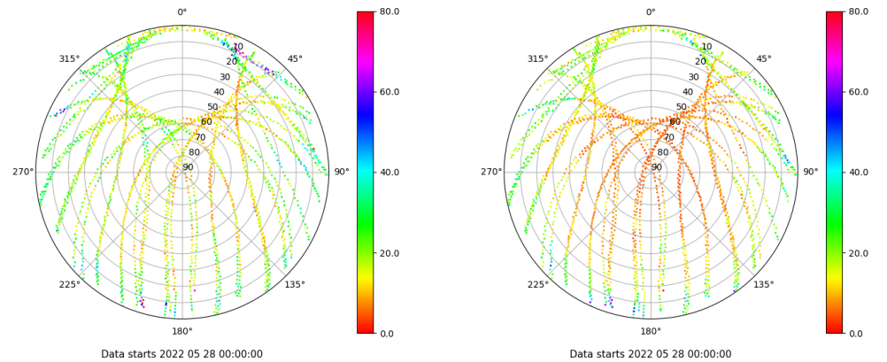
Skyplot for station VALA. Parameter M1C Data file VALA00ESP_R_2022148.xtr Skyplot for station VALA. Parameter M2C Data file VALA00ESP_R_2022148.xtr
