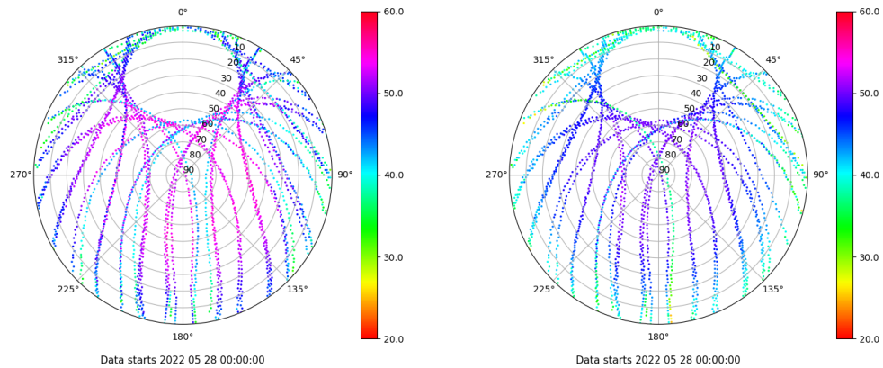
Skyplot for station VALA. Signal to Noise S1C Data file VALA00ESP_R_2022148.xtr Skyplot for station VALA. Signal to Noise S2C Data file VALA00ESP_R_2022148.xtr
