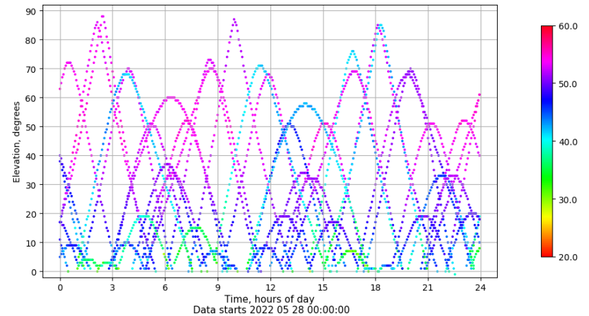
Time-elevation plot for station VALA. Signal to Noise S1C Data file VALA00ESP_R_2022148.xtr
