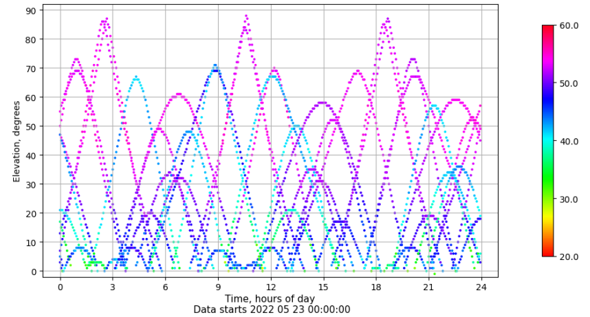
Time-elevation plot for station VALA. Signal to Noise S1C Data file VALA00ESP_R_2022143.xtr
