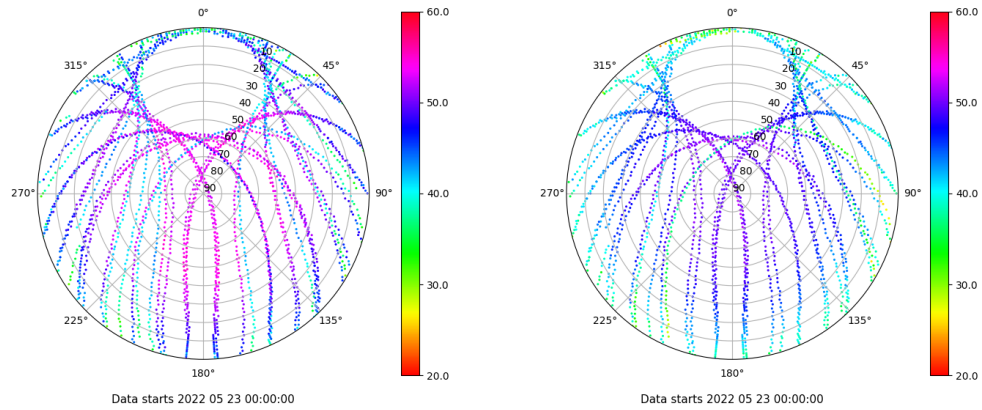
Skyplot for station VALA. Signal to Noise S1C Data file VALA00ESP_R_2022143.xtr Skyplot for station VALA. Signal to Noise S2C Data file VALA00ESP_R_2022143.xtr
