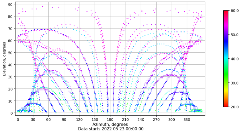
Azimuth-elevation plot for station VALA. Signal to Noise S1C Data file VALA00ESP_R_2022143.xtr
