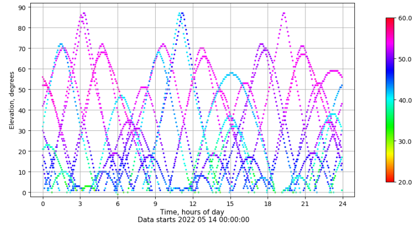
Time-elevation plot for station VALA. Signal to Noise S1C Data file VALA00ESP_R_2022134.xtr
