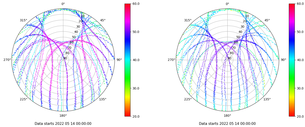
Skyplot for station VALA. Signal to Noise S1C Data file VALA00ESP_R_2022134.xtr Skyplot for station VALA. Signal to Noise S2C Data file VALA00ESP_R_2022134.xtr
