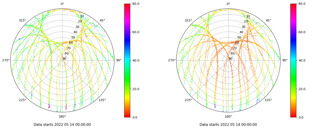
Skyplot for station VALA. Parameter M1C Data file VALA00ESP_R_2022134.xtr Skyplot for station VALA. Parameter M2C Data file VALA00ESP_R_2022134.xtr
