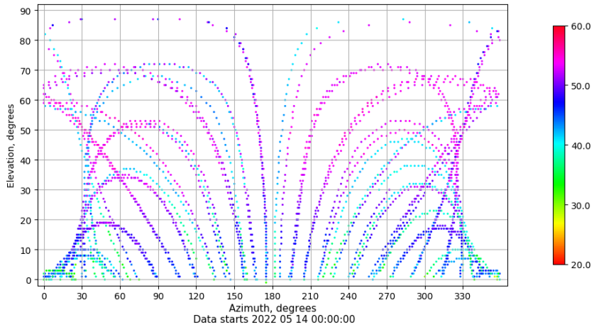
Azimuth-elevation plot for station VALA. Signal to Noise S1C Data file VALA00ESP_R_2022134.xtr
