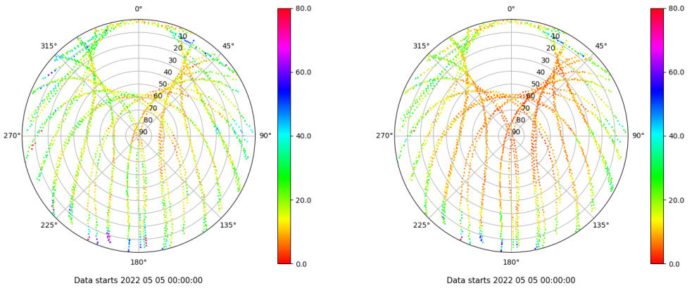
Skyplot for station VALA. Parameter M1C Data file VALA00ESP_R_2022125.xtr Skyplot for station VALA. Parameter M2C Data file VALA00ESP_R_2022125.xtr
