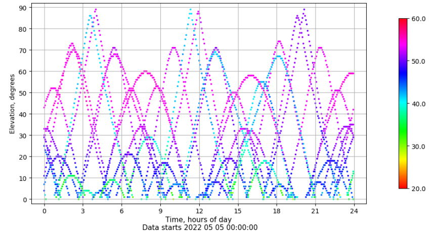
Time-elevation plot for station VALA. Signal to Noise S1C Data file VALA00ESP_R_2022125.xtr
