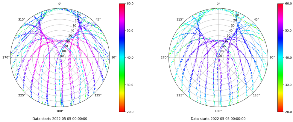
Skyplot for station VALA. Signal to Noise S1C Data file VALA00ESP_R_2022125.xtr Skyplot for station VALA. Signal to Noise S2C Data file VALA00ESP_R_2022125.xtr
