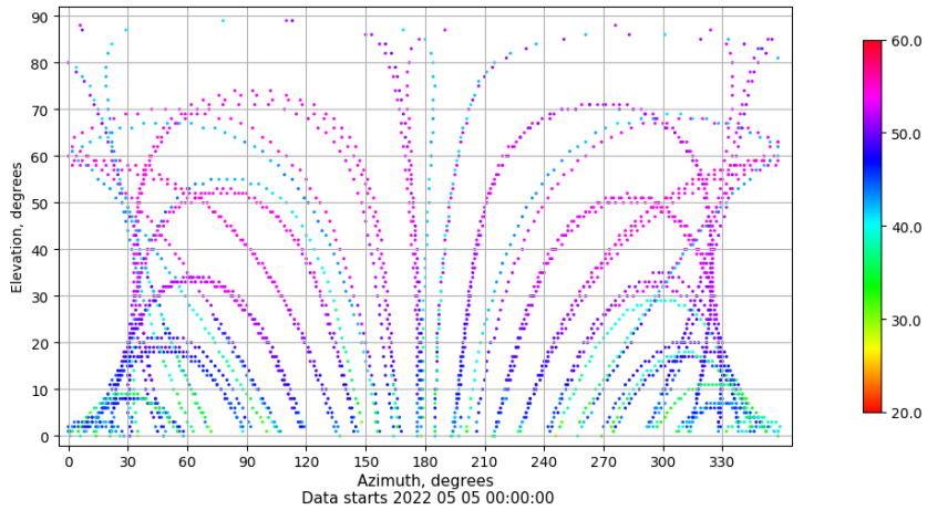
Azimuth-elevation plot for station VALA. Signal to Noise S1C Data file VALA00ESP_R_2022125.xtr
