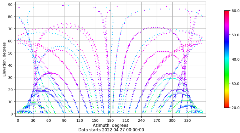
Azimuth-elevation plot for station VALA. Signal to Noise S1C Data file VALA00ESP_R_2022117.xtr
