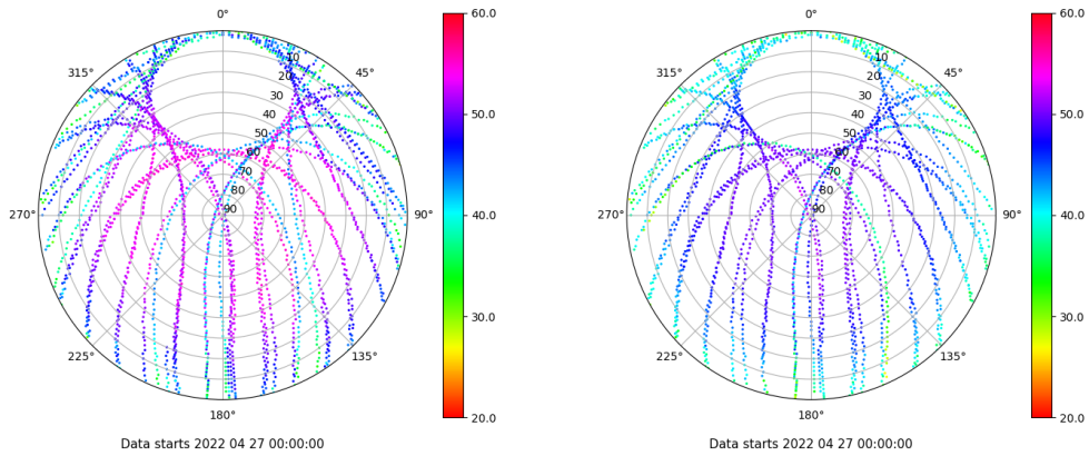
Skyplot for station VALA. Signal to Noise S1C Data file VALA00ESP_R_2022117.xtr Skyplot for station VALA. Signal to Noise S2C Data file VALA00ESP_R_2022117.xtr
