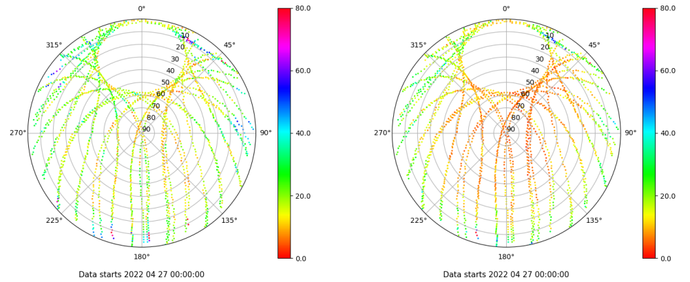
Skyplot for station VALA. Parameter M1C Data file VALA00ESP_R_2022117.xtr Skyplot for station VALA. Parameter M2C Data file VALA00ESP_R_2022117.xtr
