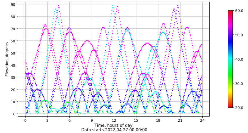
Time-elevation plot for station VALA. Signal to Noise S1C Data file VALA00ESP_R_2022117.xtr
