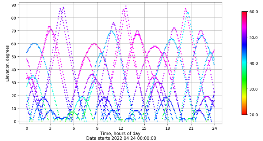
Time-elevation plot for station VALA. Signal to Noise S1C Data file VALA00ESP_R_2022114.xtr
