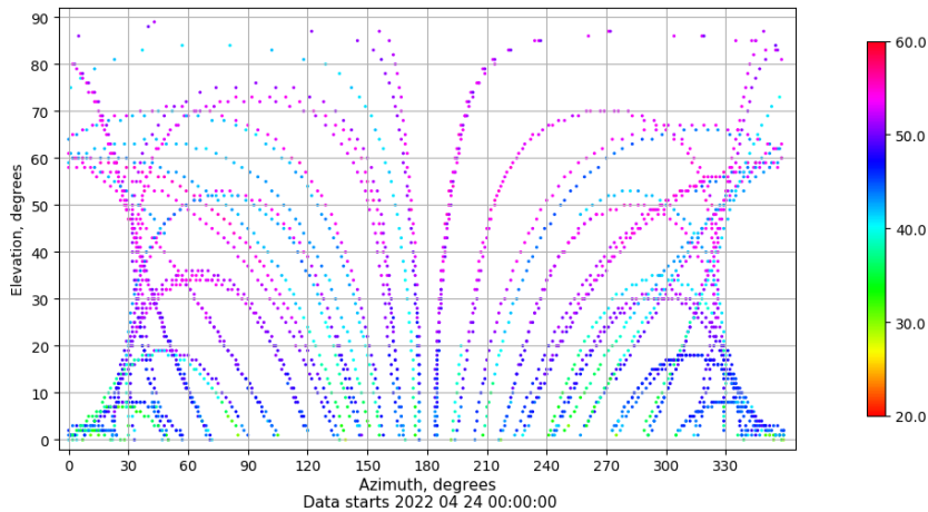
Azimuth-elevation plot for station VALA. Signal to Noise S1C Data file VALA00ESP_R_2022114.xtr
