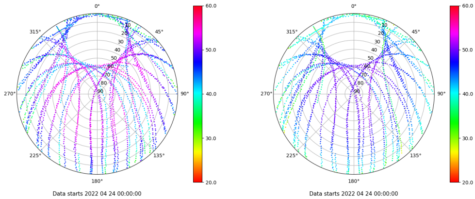
Skyplot for station VALA. Signal to Noise S1C Data file VALA00ESP_R_2022114.xtr Skyplot for station VALA. Signal to Noise S2C Data file VALA00ESP_R_2022114.xtr
