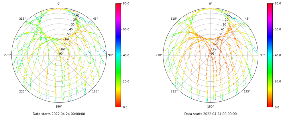
Skyplot for station VALA. Parameter M1C Data file VALA00ESP_R_2022114.xtr Skyplot for station VALA. Parameter M2C Data file VALA00ESP_R_2022114.xtr
