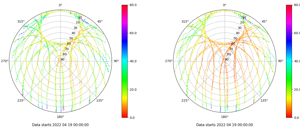
Skyplot for station VALA. Parameter M1C Data file VALA00ESP_R_2022109.xtr Skyplot for station VALA. Parameter M2C Data file VALA00ESP_R_2022109.xtr
