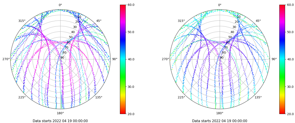
Skyplot for station VALA. Signal to Noise S1C Data file VALA00ESP_R_2022109.xtr Skyplot for station VALA. Signal to Noise S2C Data file VALA00ESP_R_2022109.xtr
