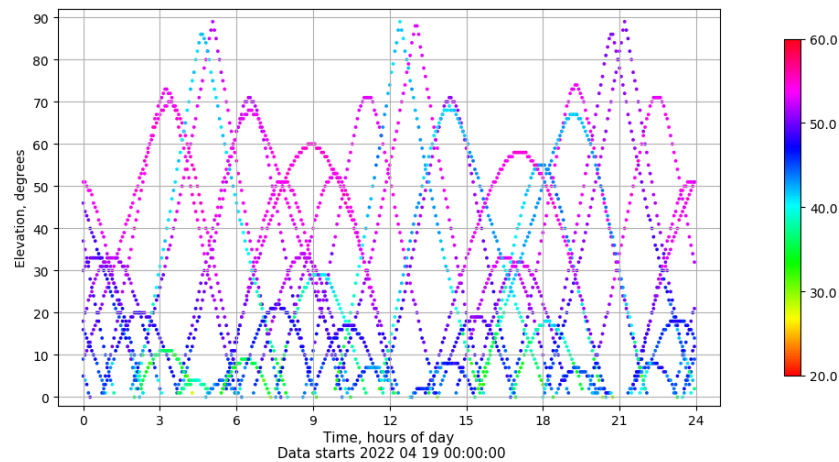
Time-elevation plot for station VALA. Signal to Noise S1C Data file VALA00ESP_R_2022109.xtr
