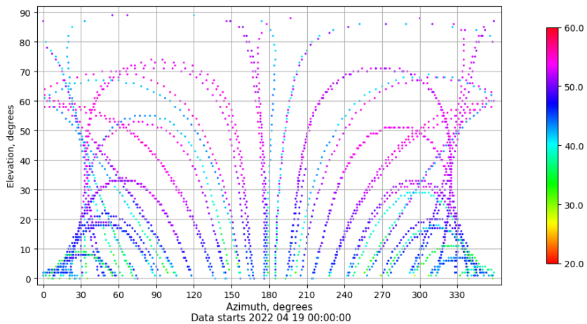
Azimuth-elevation plot for station VALA. Signal to Noise S1C Data file VALA00ESP_R_2022109.xtr
