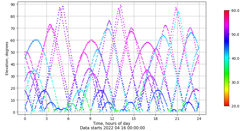
Time-elevation plot for station VALA. Signal to Noise S1C Data file VALA00ESP_R_2022106.xtr
