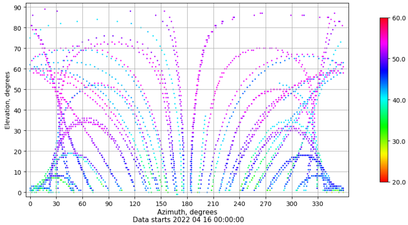
Azimuth-elevation plot for station VALA. Signal to Noise S1C Data file VALA00ESP_R_2022106.xtr
