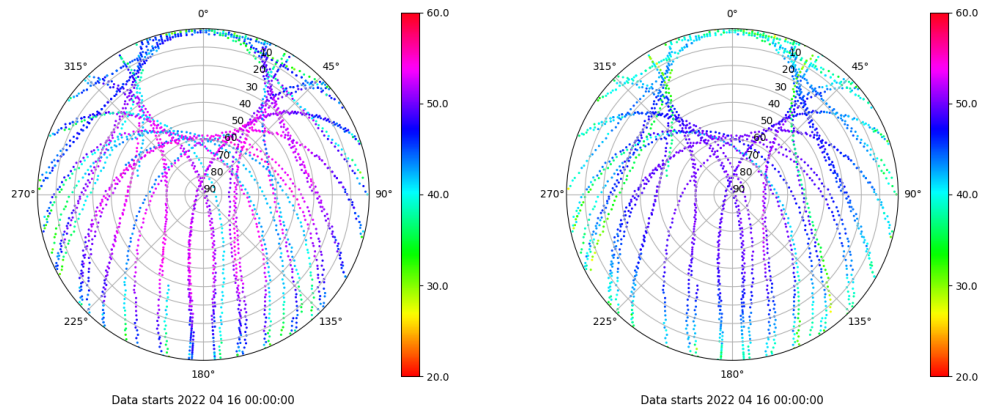
Skyplot for station VALA. Signal to Noise S1C Data file VALA00ESP_R_2022106.xtr Skyplot for station VALA. Signal to Noise S2C Data file VALA00ESP_R_2022106.xtr
