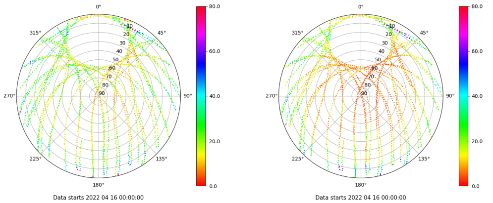
Skyplot for station VALA. Parameter M1C Data file VALA00ESP_R_2022106.xtr Skyplot for station VALA. Parameter M2C Data file VALA00ESP_R_2022106.xtr
