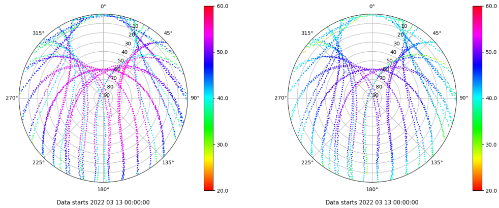
Skyplot for station VALA. Signal to Noise S1C Data file VALA00ESP_R_2022072.xtr Skyplot for station VALA. Signal to Noise S2C Data file VALA00ESP_R_2022072.xtr
