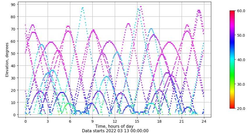
Time-elevation plot for station VALA. Signal to Noise S1C Data file VALA00ESP_R_2022072.xtr
