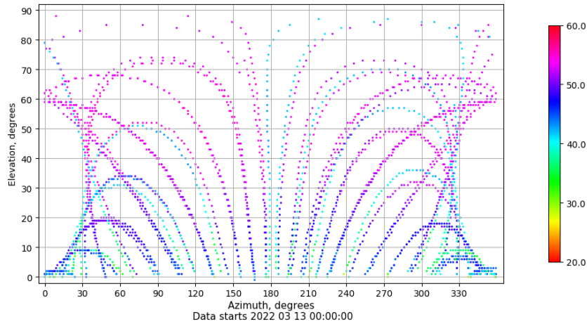
Azimuth-elevation plot for station VALA. Signal to Noise S1C Data file VALA00ESP_R_2022072.xtr
