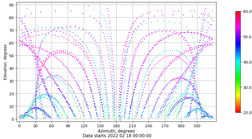
Azimuth-elevation plot for station VALA. Signal to Noise S1C Data file VALA00ESP_R_2022049.xtr
