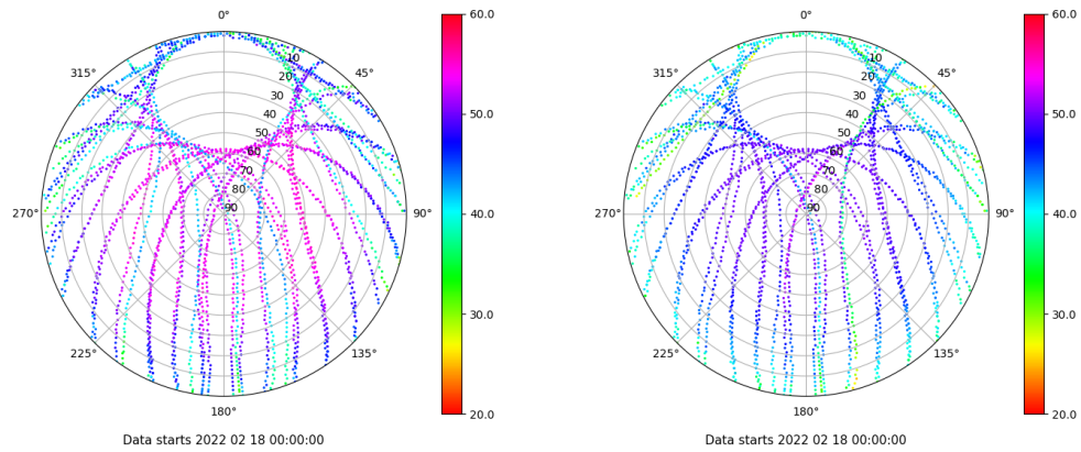
Skyplot for station VALA. Signal to Noise S1C Data file VALA00ESP_R_2022049.xtr Skyplot for station VALA. Signal to Noise S2C Data file VALA00ESP_R_2022049.xtr
