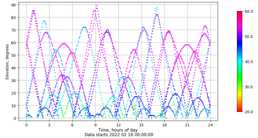
Time-elevation plot for station VALA. Signal to Noise S1C Data file VALA00ESP_R_2022049.xtr
