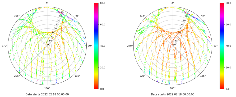
Skyplot for station VALA. Parameter M1C Data file VALA00ESP_R_2022049.xtr Skyplot for station VALA. Parameter M2C Data file VALA00ESP_R_2022049.xtr
