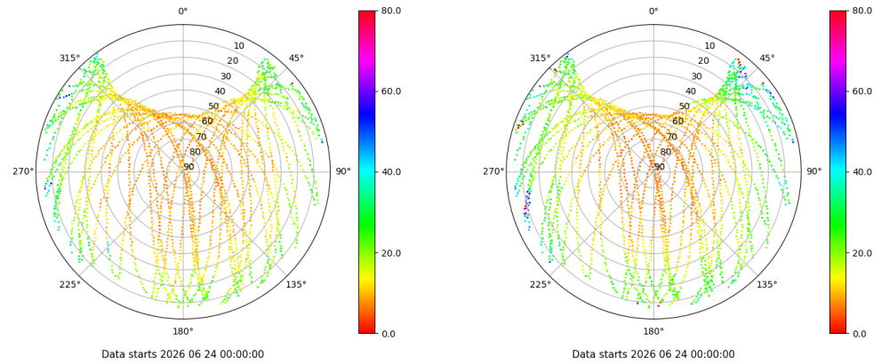
Skyplot for station ULP2. Parameter M1C Data file ULP200ESP_R_2026175.xtr Skyplot for station ULP2. Parameter M2X Data file ULP200ESP_R_2026175.xtr
