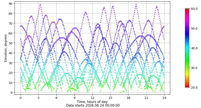
Time-elevation plot for station ULP2. Signal to Noise S1C Data file ULP200ESP_R_2026175.xtr
