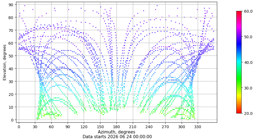
Azimuth-elevation plot for station ULP2. Signal to Noise S1C Data file ULP200ESP_R_2026175.xtr
