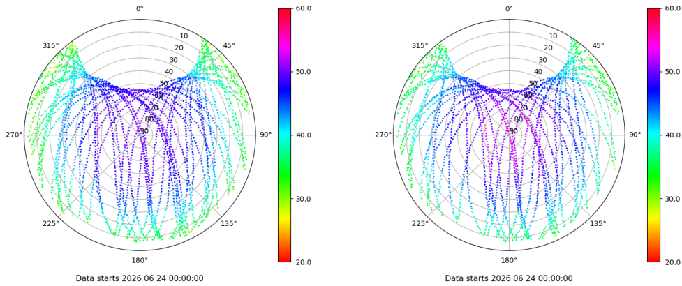
Skyplot for station ULP2. Signal to Noise S1C Data file ULP200ESP_R_2026175.xtr Skyplot for station ULP2. Signal to Noise S2X Data file ULP200ESP_R_2026175.xtr
