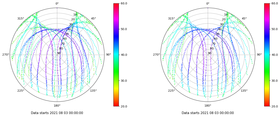
Skyplot for station ULP2. Signal to Noise S1C Data file ULP200ESP_R_2021215.xtr Skyplot for station ULP2. Signal to Noise S2C Data file ULP200ESP_R_2021215.xtr
