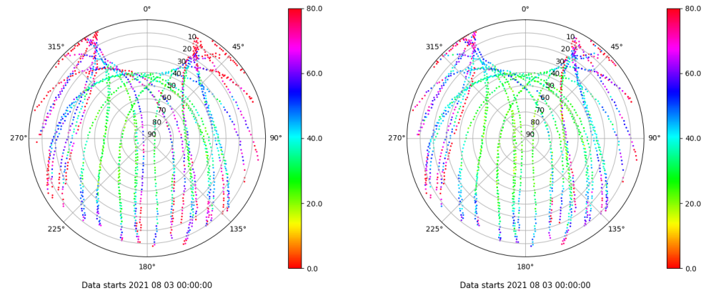
Skyplot for station ULP2. Parameter M1C Data file ULP200ESP_R_2021215.xtr Skyplot for station ULP2. Parameter M2C Data file ULP200ESP_R_2021215.xtr
