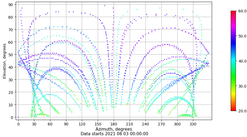
Azimuth-elevation plot for station ULP2. Signal to Noise S1C Data file ULP200ESP_R_2021215.xtr
