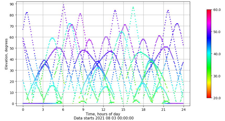
Time-elevation plot for station ULP2. Signal to Noise S1C Data file ULP200ESP_R_2021215.xtr
