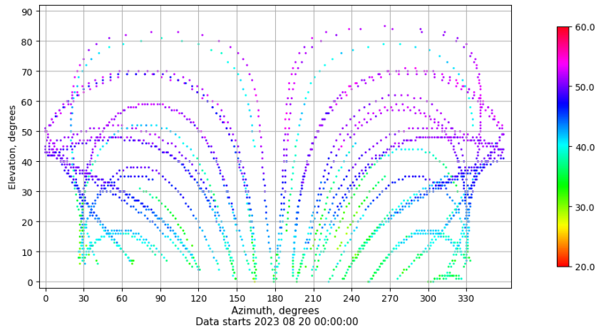
Azimuth-elevation plot for station TN03. Signal to Noise S1C Data file TN0300ESP_R_2023232.xtr
