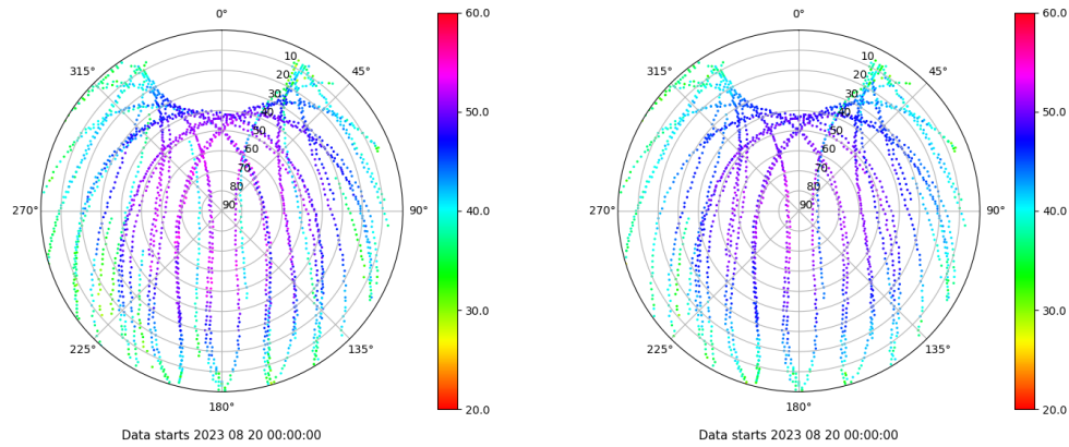
Skyplot for station TN03. Signal to Noise S1C Data file TN0300ESP_R_2023232.xtr Skyplot for station TN03. Signal to Noise S2C Data file TN0300ESP_R_2023232.xtr
