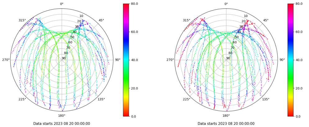
Skyplot for station TN03. Parameter M1C Data file TN0300ESP_R_2023232.xtr Skyplot for station TN03. Parameter M2C Data file TN0300ESP_R_2023232.xtr
