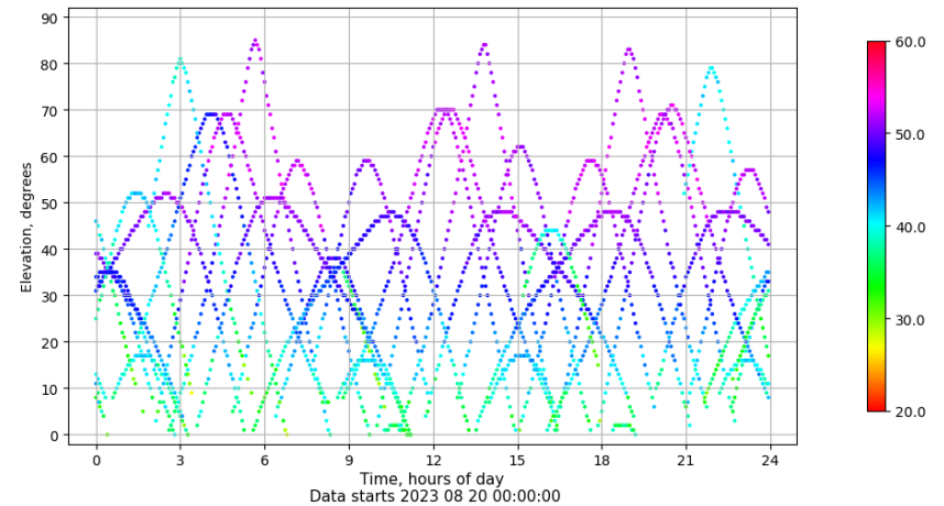
Time-elevation plot for station TN03. Signal to Noise S1C Data file TN0300ESP_R_2023232.xtr
