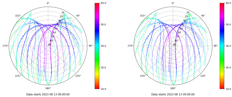
Skyplot for station TN03. Signal to Noise S1C Data file TN0300ESP_R_2023225.xtr Skyplot for station TN03. Signal to Noise S2C Data file TN0300ESP_R_2023225.xtr
