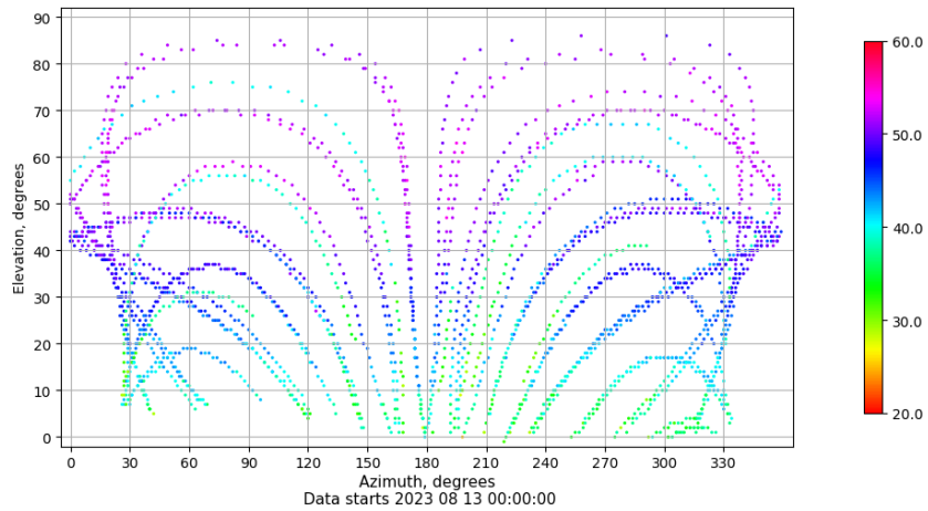
Azimuth-elevation plot for station TN03. Signal to Noise S1C Data file TN0300ESP_R_2023225.xtr
