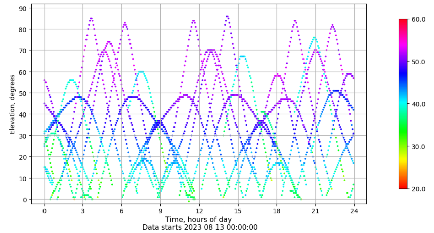
Time-elevation plot for station TN03. Signal to Noise S1C Data file TN0300ESP_R_2023225.xtr
