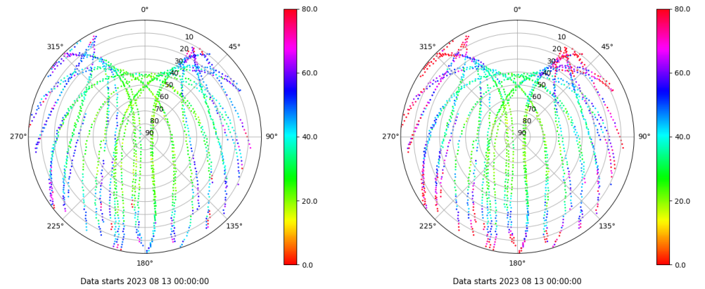
Skyplot for station TN03. Parameter M1C Data file TN0300ESP_R_2023225.xtr Skyplot for station TN03. Parameter M2C Data file TN0300ESP_R_2023225.xtr
