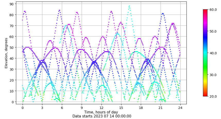
Time-elevation plot for station TN03. Signal to Noise S1C Data file TN0300ESP_R_2023195.xtr
