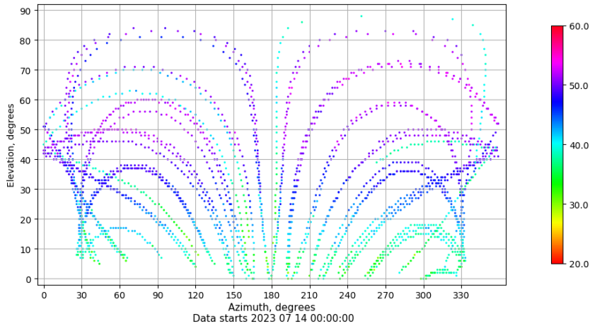
Azimuth-elevation plot for station TN03. Signal to Noise S1C Data file TN0300ESP_R_2023195.xtr
