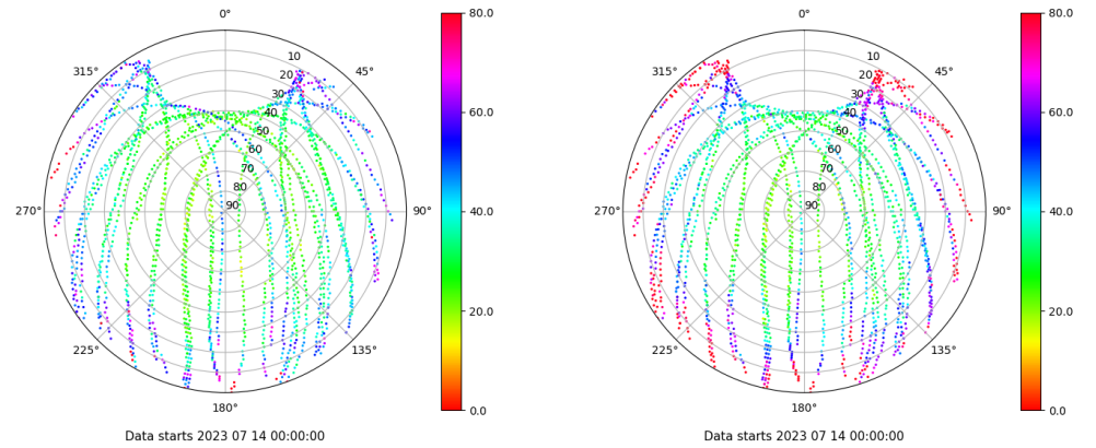
Skyplot for station TN03. Parameter M1C Data file TN0300ESP_R_2023195.xtr Skyplot for station TN03. Parameter M2C Data file TN0300ESP_R_2023195.xtr
