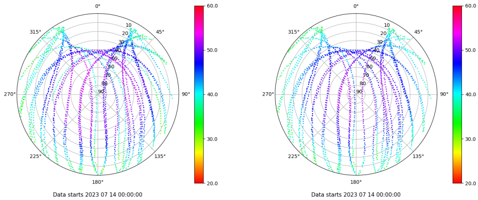
Skyplot for station TN03. Signal to Noise S1C Data file TN0300ESP_R_2023195.xtr Skyplot for station TN03. Signal to Noise S2C Data file TN0300ESP_R_2023195.xtr
