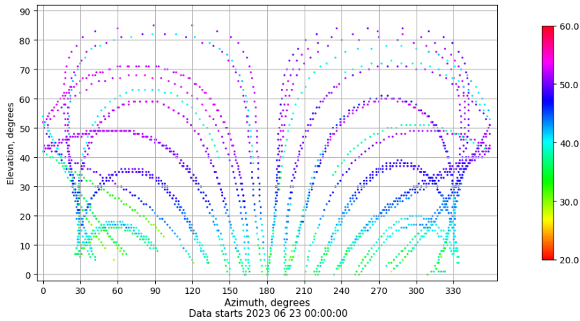
Azimuth-elevation plot for station TN03. Signal to Noise S1C Data file TN0300ESP_R_2023174.xtr
