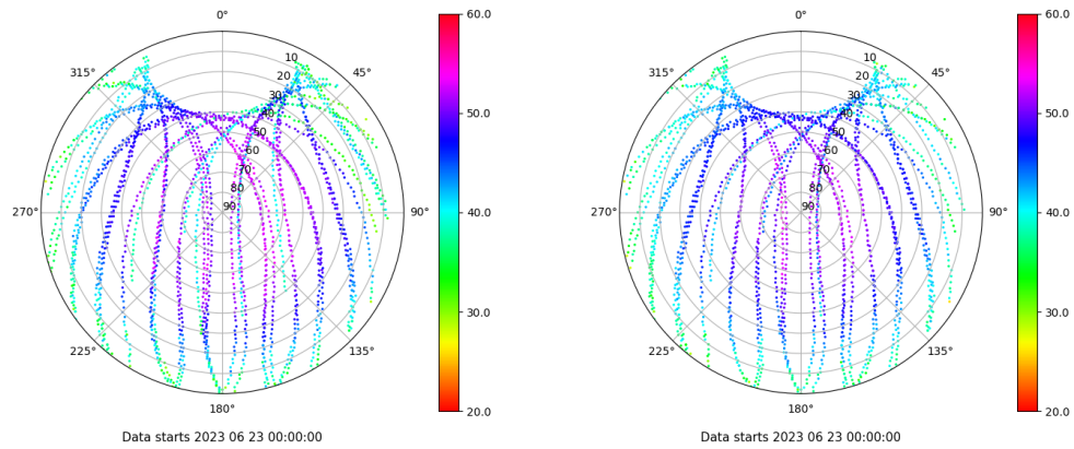
Skyplot for station TN03. Signal to Noise S1C Data file TN0300ESP_R_2023174.xtr Skyplot for station TN03. Signal to Noise S2C Data file TN0300ESP_R_2023174.xtr
