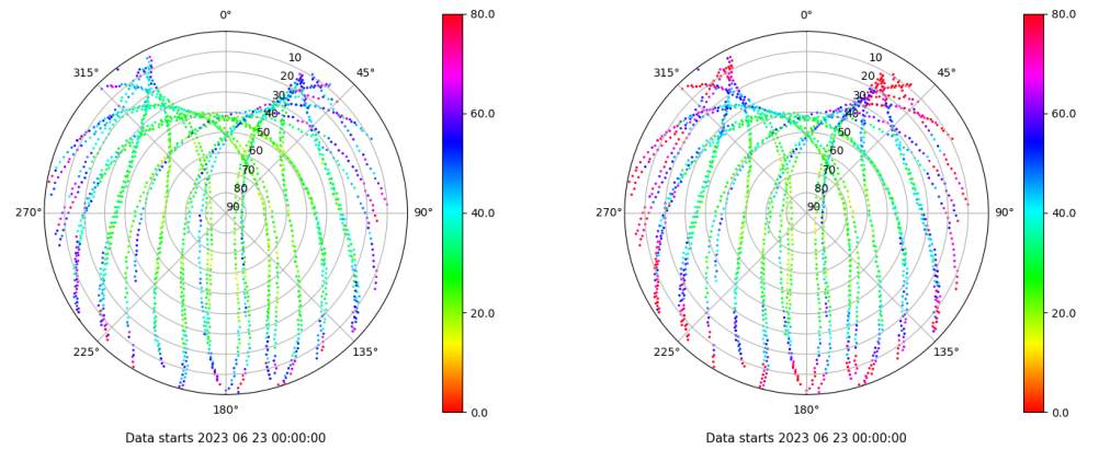
Skyplot for station TN03. Parameter M1C Data file TN0300ESP_R_2023174.xtr Skyplot for station TN03. Parameter M2C Data file TN0300ESP_R_2023174.xtr
