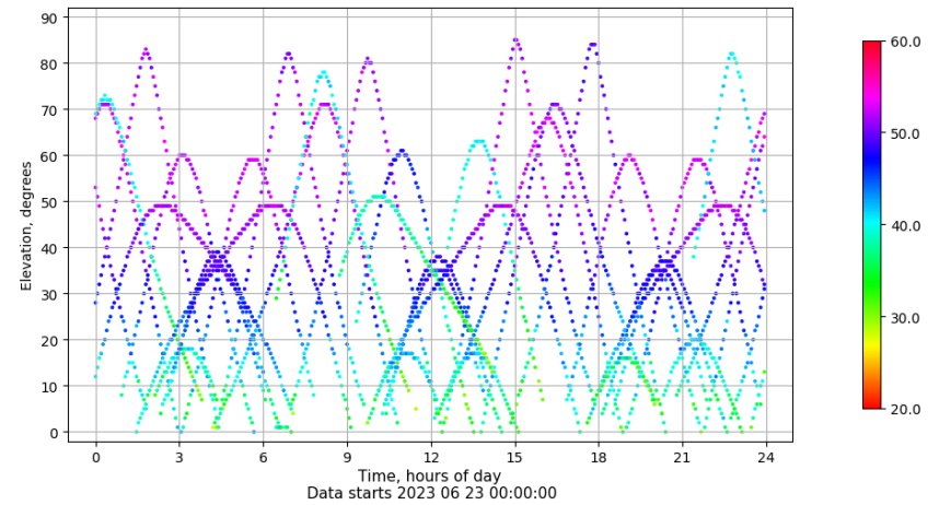
Time-elevation plot for station TN03. Signal to Noise S1C Data file TN0300ESP_R_2023174.xtr
