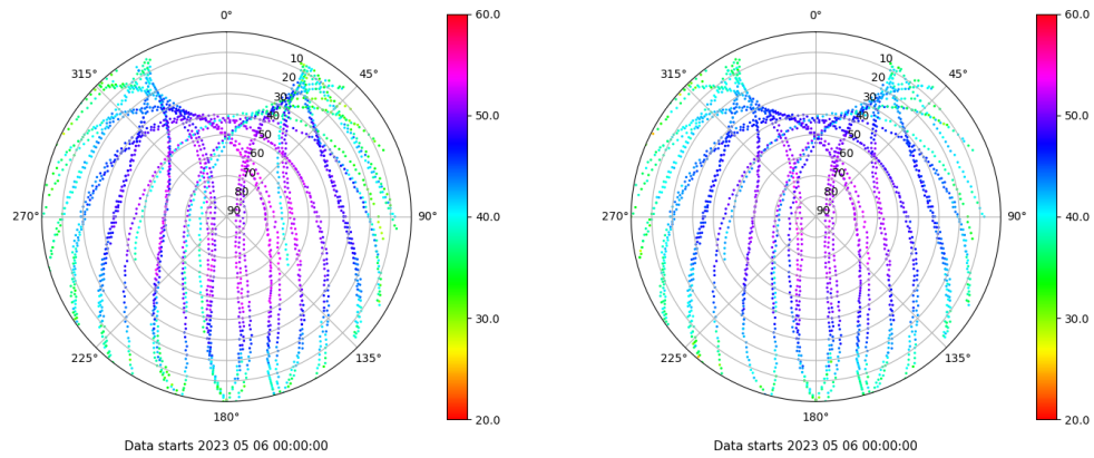
Skyplot for station TN03. Signal to Noise S1C Data file TN0300ESP_R_2023126.xtr Skyplot for station TN03. Signal to Noise S2C Data file TN0300ESP_R_2023126.xtr
