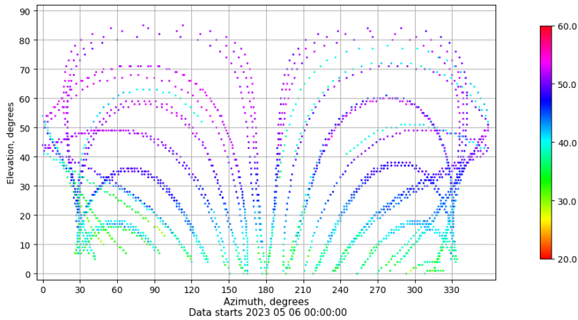
Azimuth-elevation plot for station TN03. Signal to Noise S1C Data file TN0300ESP_R_2023126.xtr
