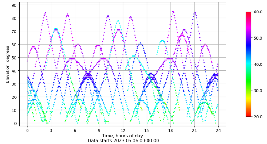
Time-elevation plot for station TN03. Signal to Noise S1C Data file TN0300ESP_R_2023126.xtr
