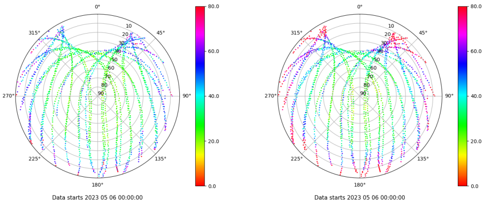
Skyplot for station TN03. Parameter M1C Data file TN0300ESP_R_2023126.xtr Skyplot for station TN03. Parameter M2C Data file TN0300ESP_R_2023126.xtr
