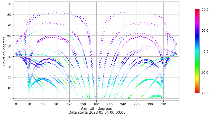
Azimuth-elevation plot for station TN03. Signal to Noise S1C Data file TN0300ESP_R_2023124.xtr
