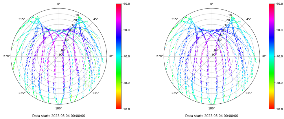
Skyplot for station TN03. Signal to Noise S1C Data file TN0300ESP_R_2023124.xtr Skyplot for station TN03. Signal to Noise S2C Data file TN0300ESP_R_2023124.xtr
