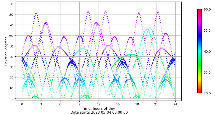
Time-elevation plot for station TN03. Signal to Noise S1C Data file TN0300ESP_R_2023124.xtr
