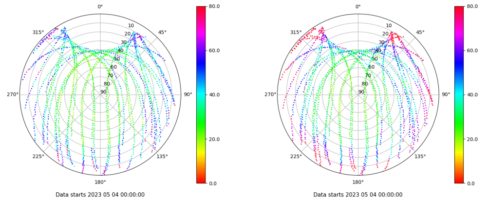
Skyplot for station TN03. Parameter M1C Data file TN0300ESP_R_2023124.xtr Skyplot for station TN03. Parameter M2C Data file TN0300ESP_R_2023124.xtr
