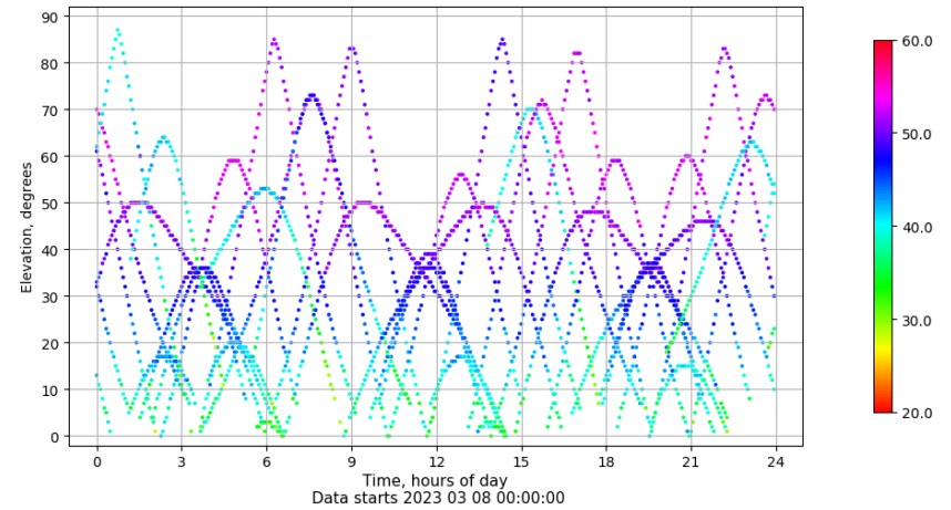
Time-elevation plot for station TN03. Signal to Noise S1C Data file TN0300ESP_R_2023067.xtr
