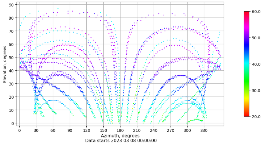
Azimuth-elevation plot for station TN03. Signal to Noise S1C Data file TN0300ESP_R_2023067.xtr
