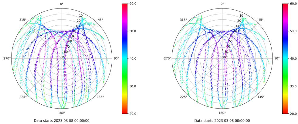
Skyplot for station TN03. Signal to Noise S1C Data file TN0300ESP_R_2023067.xtr Skyplot for station TN03. Signal to Noise S2C Data file TN0300ESP_R_2023067.xtr
