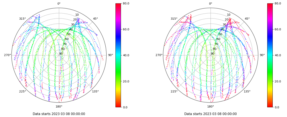
Skyplot for station TN03. Parameter M1C Data file TN0300ESP_R_2023067.xtr Skyplot for station TN03. Parameter M2C Data file TN0300ESP_R_2023067.xtr
