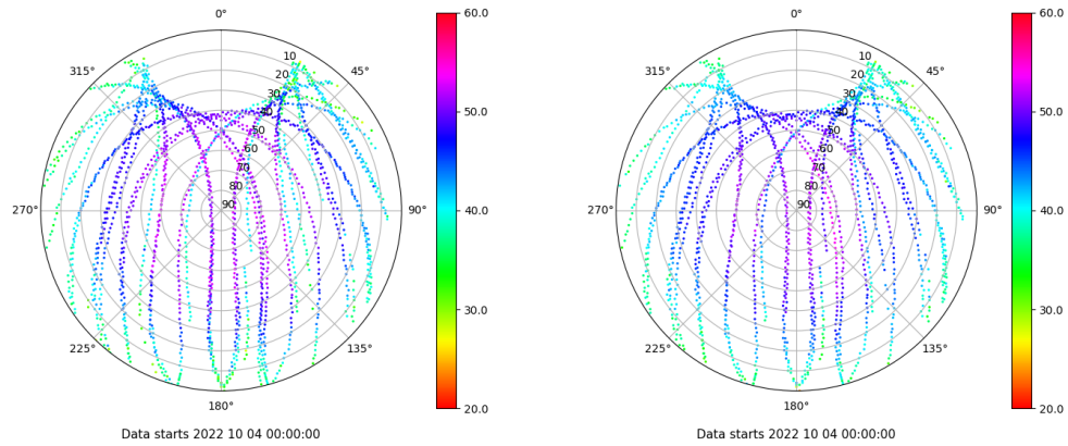
Skyplot for station TN03. Signal to Noise S1C Data file TN0300ESP_R_2022277.xtr Skyplot for station TN03. Signal to Noise S2C Data file TN0300ESP_R_2022277.xtr
