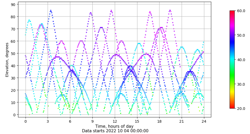
Time-elevation plot for station TN03. Signal to Noise S1C Data file TN0300ESP_R_2022277.xtr
