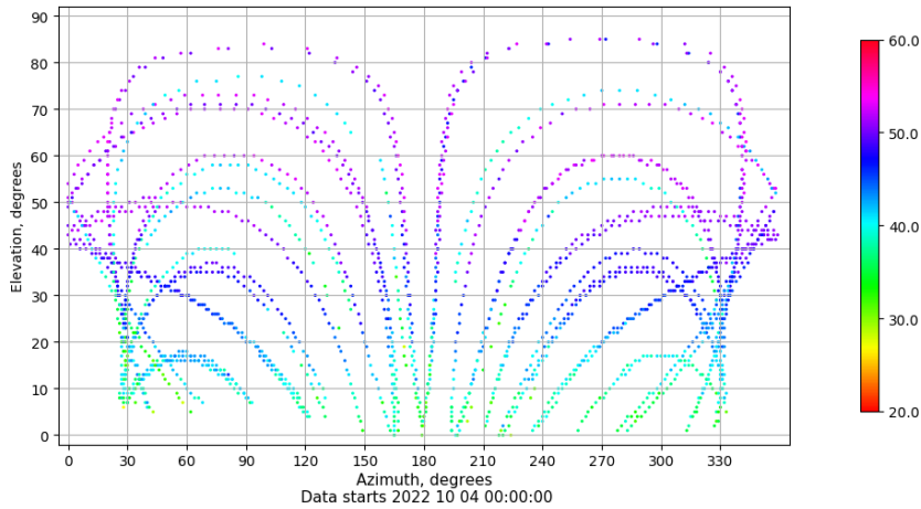
Azimuth-elevation plot for station TN03. Signal to Noise S1C Data file TN0300ESP_R_2022277.xtr
