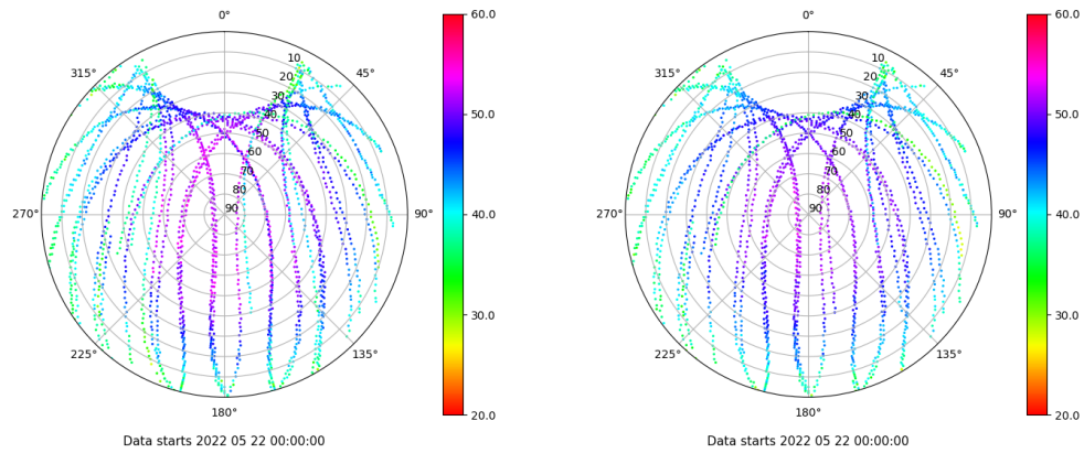
Skyplot for station TN03. Signal to Noise S1C Data file TN0300ESP_R_2022142.xtr Skyplot for station TN03. Signal to Noise S2C Data file TN0300ESP_R_2022142.xtr
