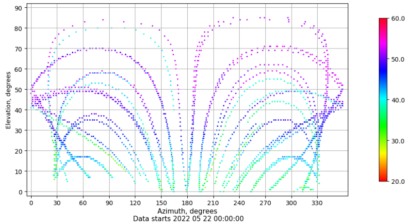
Azimuth-elevation plot for station TN03. Signal to Noise S1C Data file TN0300ESP_R_2022142.xtr
