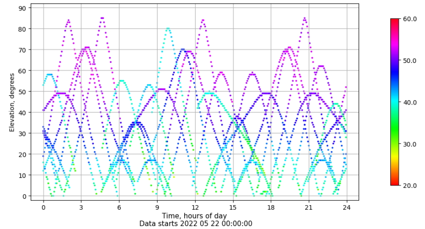
Time-elevation plot for station TN03. Signal to Noise S1C Data file TN0300ESP_R_2022142.xtr
