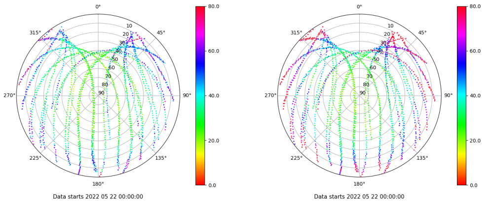
Skyplot for station TN03. Parameter M1C Data file TN0300ESP_R_2022142.xtr Skyplot for station TN03. Parameter M2C Data file TN0300ESP_R_2022142.xtr
