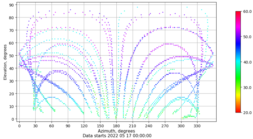
Azimuth-elevation plot for station TN03. Signal to Noise S1C Data file TN0300ESP_R_2022137.xtr
