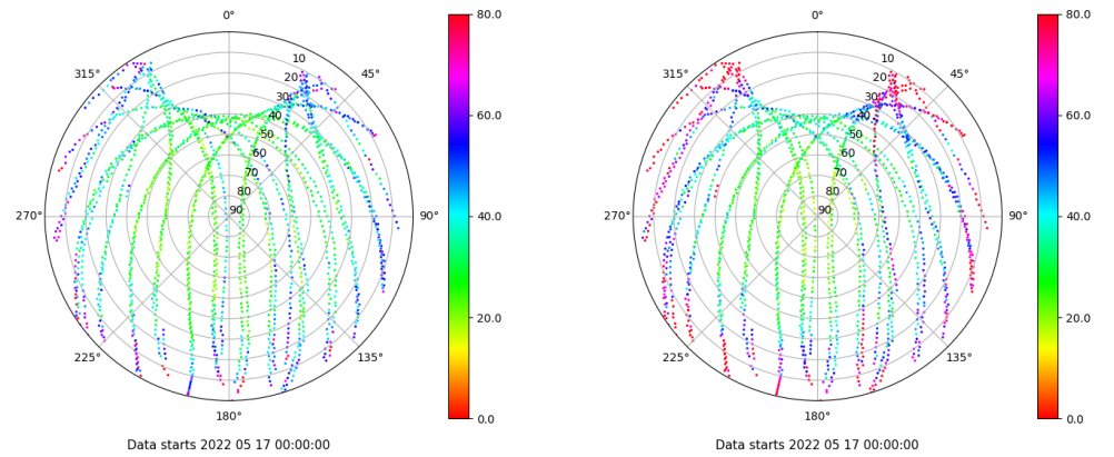
Skyplot for station TN03. Parameter M1C Data file TN0300ESP_R_2022137.xtr Skyplot for station TN03. Parameter M2C Data file TN0300ESP_R_2022137.xtr
