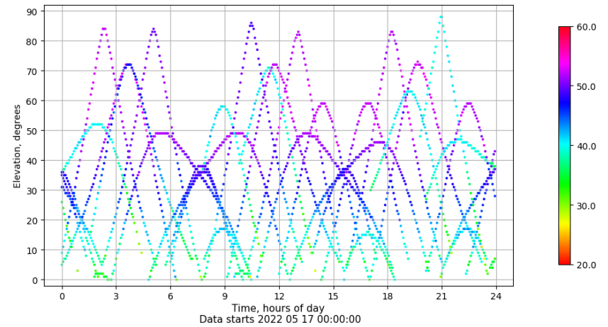
Time-elevation plot for station TN03. Signal to Noise S1C Data file TN0300ESP_R_2022137.xtr
