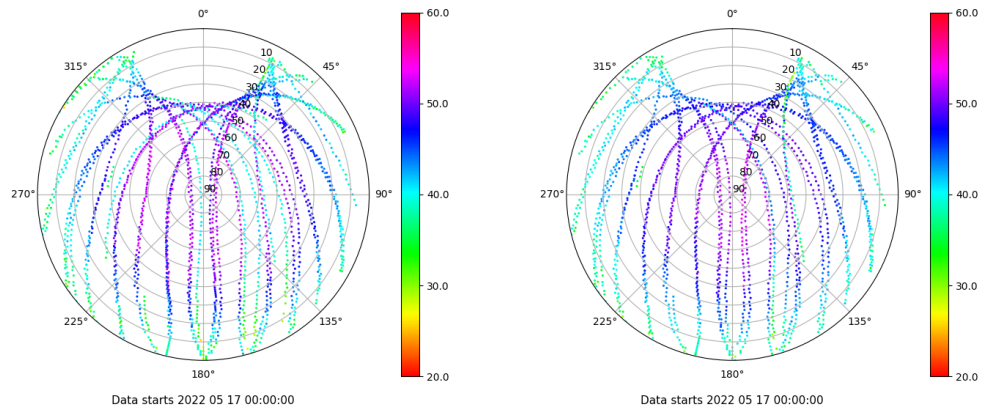
Skyplot for station TN03. Signal to Noise S1C Data file TN0300ESP_R_2022137.xtr Skyplot for station TN03. Signal to Noise S2C Data file TN0300ESP_R_2022137.xtr
