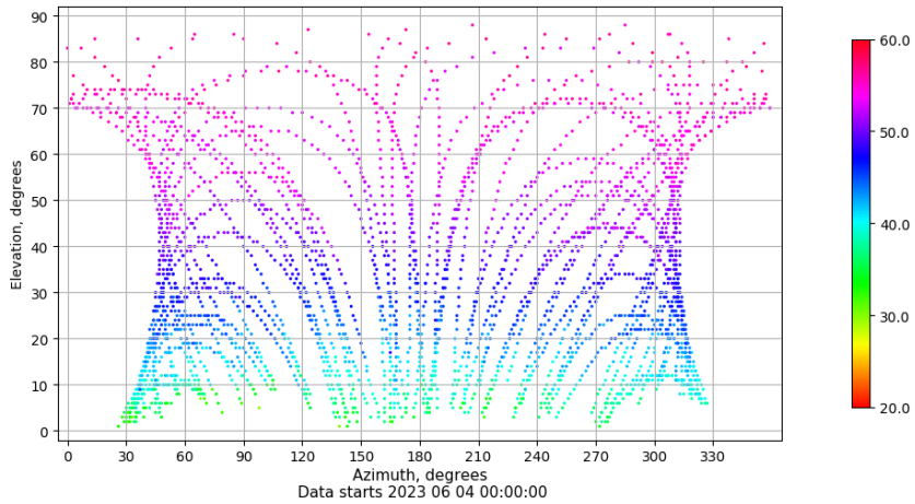
Azimuth-elevation plot for station TERU. Signal to Noise S1C Data file TERU00ESP_R_2023155.xtr
