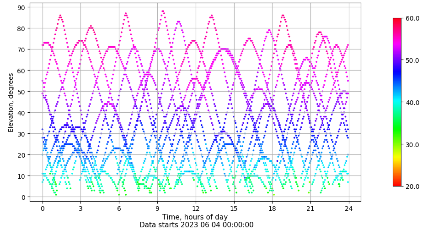
Time-elevation plot for station TERU. Signal to Noise S1C Data file TERU00ESP_R_2023155.xtr
