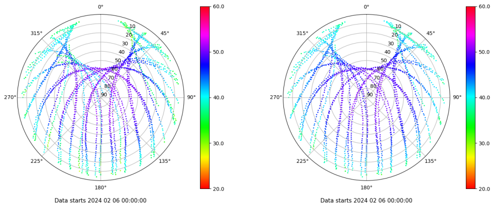
Skyplot for station TARR. Signal to Noise S1C Data file TARR00ESP_R_2024037.xtr Skyplot for station TARR. Signal to Noise S2P Data file TARR00ESP_R_2024037.xtr
