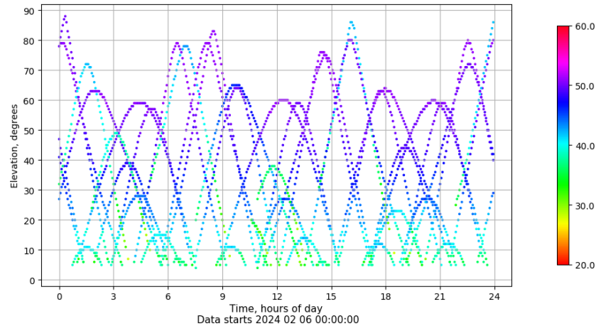
Time-elevation plot for station TARR. Signal to Noise S1C Data file TARR00ESP_R_2024037.xtr
