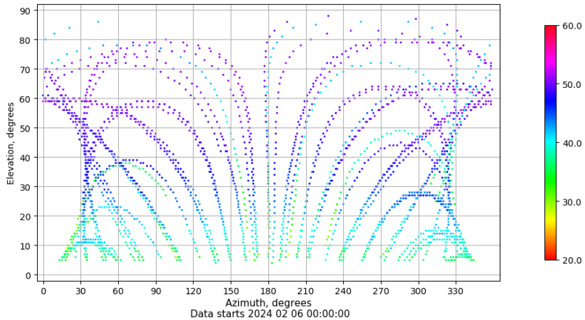
Azimuth-elevation plot for station TARR. Signal to Noise S1C Data file TARR00ESP_R_2024037.xtr
