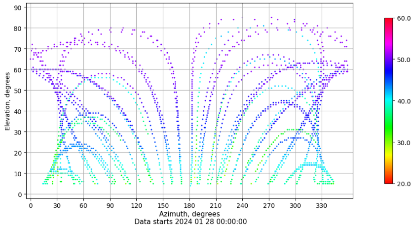
Azimuth-elevation plot for station TARR. Signal to Noise S1C Data file TARR00ESP_R_2024028.xtr
