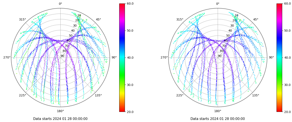
Skyplot for station TARR. Signal to Noise S1C Data file TARR00ESP_R_2024028.xtr Skyplot for station TARR. Signal to Noise S2P Data file TARR00ESP_R_2024028.xtr
