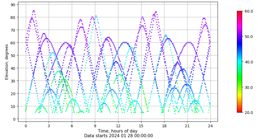
Time-elevation plot for station TARR. Signal to Noise S1C Data file TARR00ESP_R_2024028.xtr
