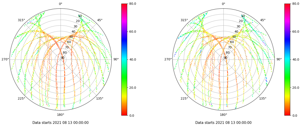
Skyplot for station TAR0. Parameter M1C Data file TAR000ESP_R_2021225.xtr Skyplot for station TAR0. Parameter M2P Data file TAR000ESP_R_2021225.xtr
