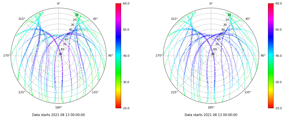
Skyplot for station TAR0. Signal to Noise S1C Data file TAR000ESP_R_2021225.xtr Skyplot for station TAR0. Signal to Noise S2P Data file TAR000ESP_R_2021225.xtr
