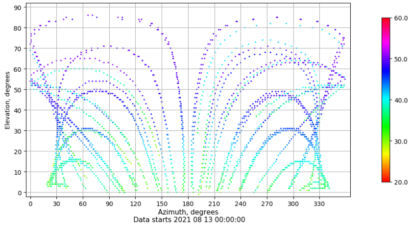
Azimuth-elevation plot for station TAR0. Signal to Noise S1C Data file TAR000ESP_R_2021225.xtr
