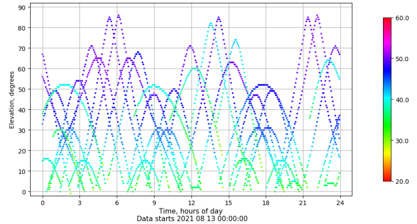
Time-elevation plot for station TAR0. Signal to Noise S1C Data file TAR000ESP_R_2021225.xtr
