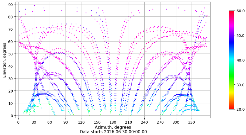
Azimuth-elevation plot for station TALV. Signal to Noise S1C Data file TALV00ESP_R_2026181.xtr
