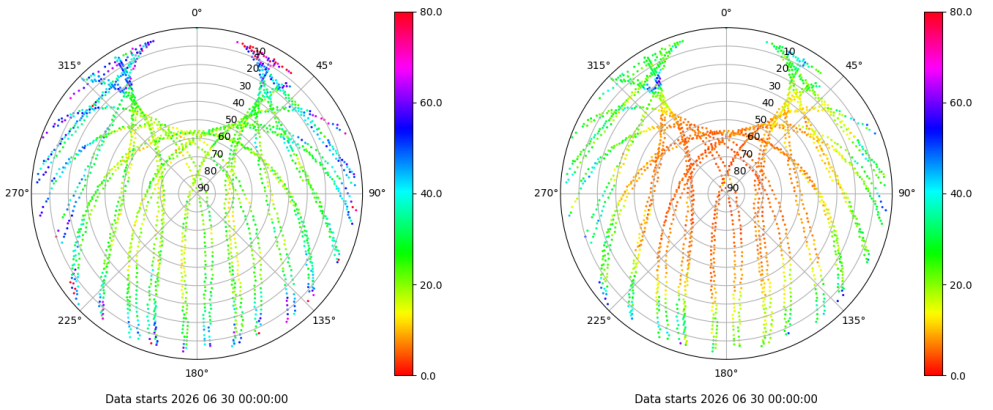
Skyplot for station TALV. Parameter M1C Data file TALV00ESP_R_2026181.xtr Skyplot for station TALV. Parameter M2P Data file TALV00ESP_R_2026181.xtr
