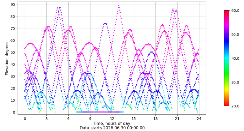
Time-elevation plot for station TALV. Signal to Noise S1C Data file TALV00ESP_R_2026181.xtr
