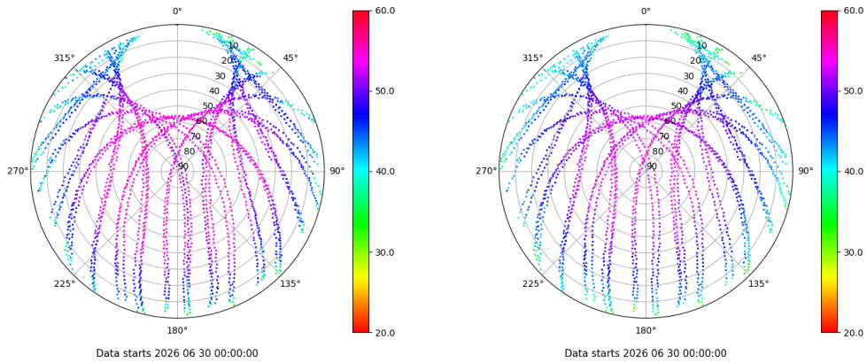
Skyplot for station TALV. Signal to Noise S1C Data file TALV00ESP_R_2026181.xtr Skyplot for station TALV. Signal to Noise S2P Data file TALV00ESP_R_2026181.xtr
