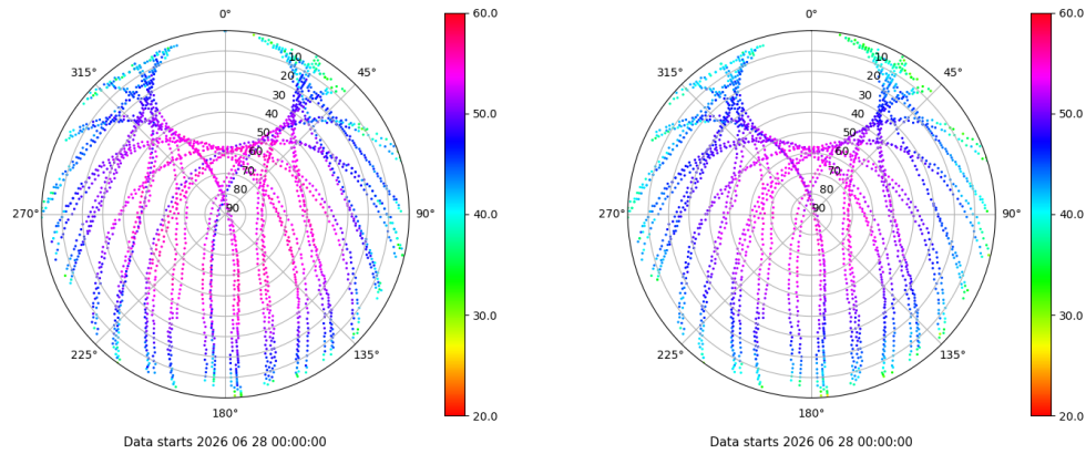
Skyplot for station TALV. Signal to Noise S1C Data file TALV00ESP_R_2026179.xtr Skyplot for station TALV. Signal to Noise S2P Data file TALV00ESP_R_2026179.xtr
