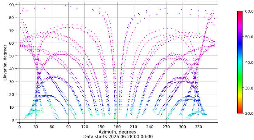
Azimuth-elevation plot for station TALV. Signal to Noise S1C Data file TALV00ESP_R_2026179.xtr
