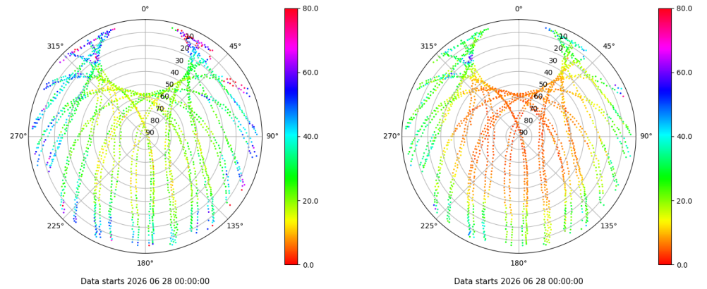
Skyplot for station TALV. Parameter M1C Data file TALV00ESP_R_2026179.xtr Skyplot for station TALV. Parameter M2P Data file TALV00ESP_R_2026179.xtr
