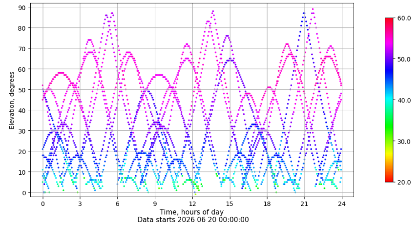
Time-elevation plot for station TALV. Signal to Noise S1C Data file TALV00ESP_R_2026171.xtr
