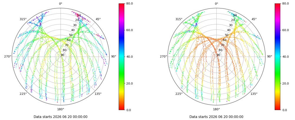
Skyplot for station TALV. Parameter M1C Data file TALV00ESP_R_2026171.xtr Skyplot for station TALV. Parameter M2P Data file TALV00ESP_R_2026171.xtr
