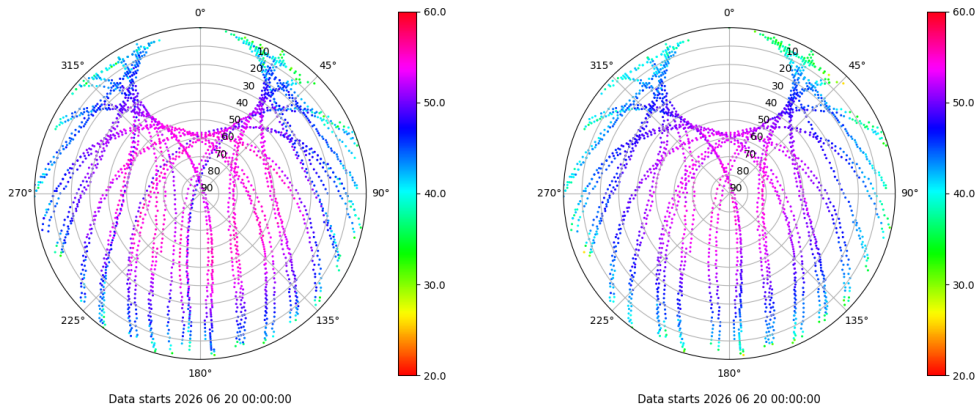
Skyplot for station TALV. Signal to Noise S1C Data file TALV00ESP_R_2026171.xtr Skyplot for station TALV. Signal to Noise S2P Data file TALV00ESP_R_2026171.xtr
