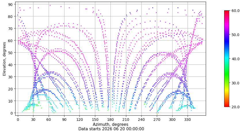
Azimuth-elevation plot for station TALV. Signal to Noise S1C Data file TALV00ESP_R_2026171.xtr
