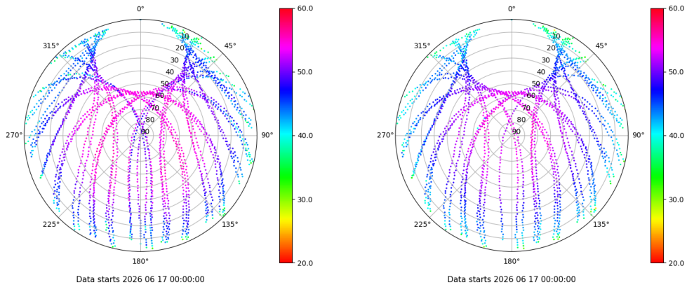
Skyplot for station TALV. Signal to Noise S1C Data file TALV00ESP_R_2026168.xtr Skyplot for station TALV. Signal to Noise S2P Data file TALV00ESP_R_2026168.xtr
