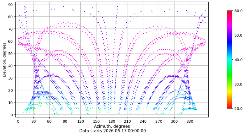
Azimuth-elevation plot for station TALV. Signal to Noise S1C Data file TALV00ESP_R_2026168.xtr
