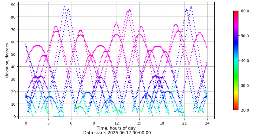
Time-elevation plot for station TALV. Signal to Noise S1C Data file TALV00ESP_R_2026168.xtr
