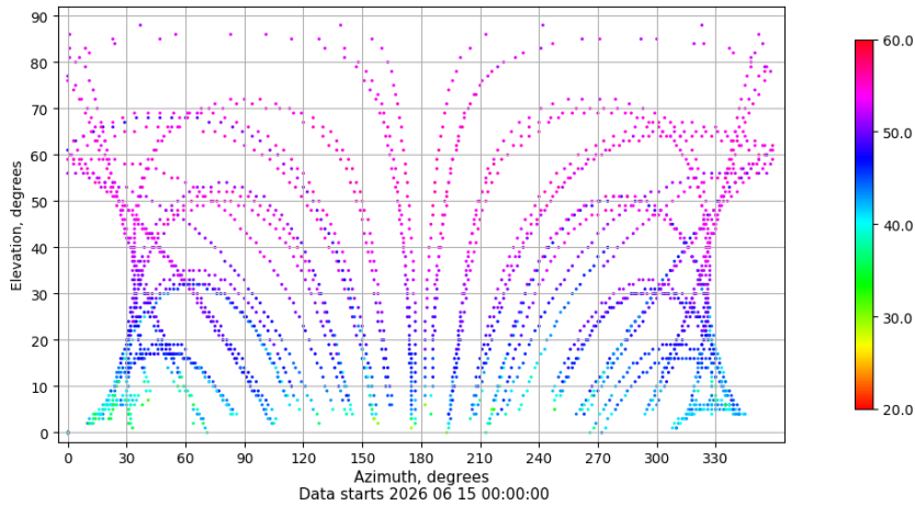
Azimuth-elevation plot for station TALV. Signal to Noise S1C Data file TALV00ESP_R_2026166.xtr
