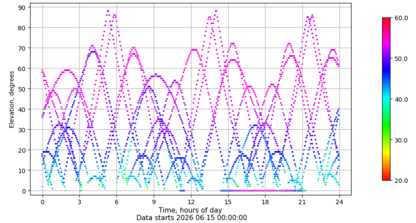
Time-elevation plot for station TALV. Signal to Noise S1C Data file TALV00ESP_R_2026166.xtr
