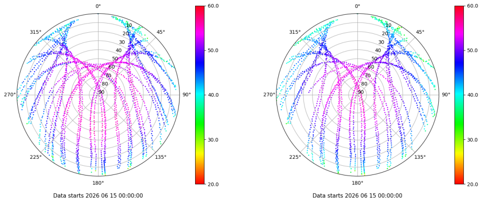
Skyplot for station TALV. Signal to Noise S1C Data file TALV00ESP_R_2026166.xtr Skyplot for station TALV. Signal to Noise S2P Data file TALV00ESP_R_2026166.xtr
